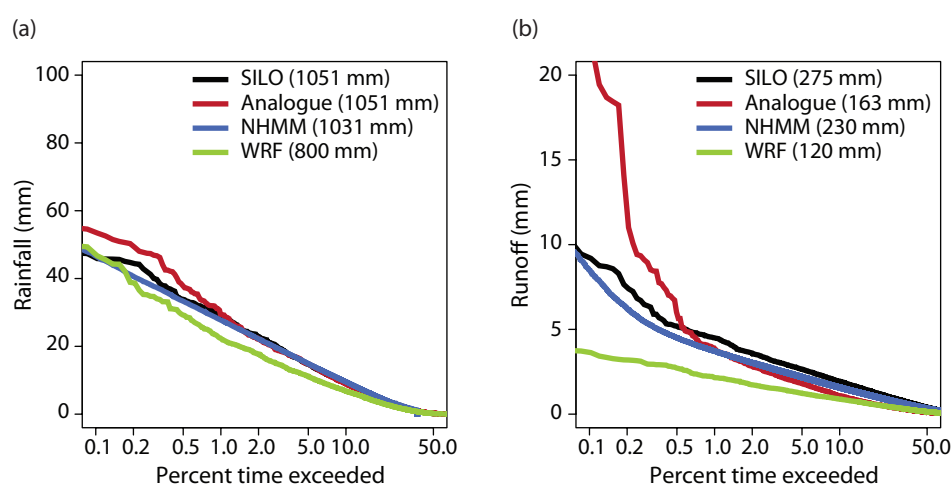
Figure 15. Modelled versus observed (SILO) daily (a) rainfall and (b) runoff distribution (1985–2000) for the Yea River at Devlins Bridge. Daily rainfall is derived from analogue downscaling (bias corrected) NHMM statistical downscaling (fitted to observed rainfall), and WRF dynamical downscaling (non bias corrected) models. Mean annual rainfall and runoff are shown in brackets after the name of the downscaling approach.
