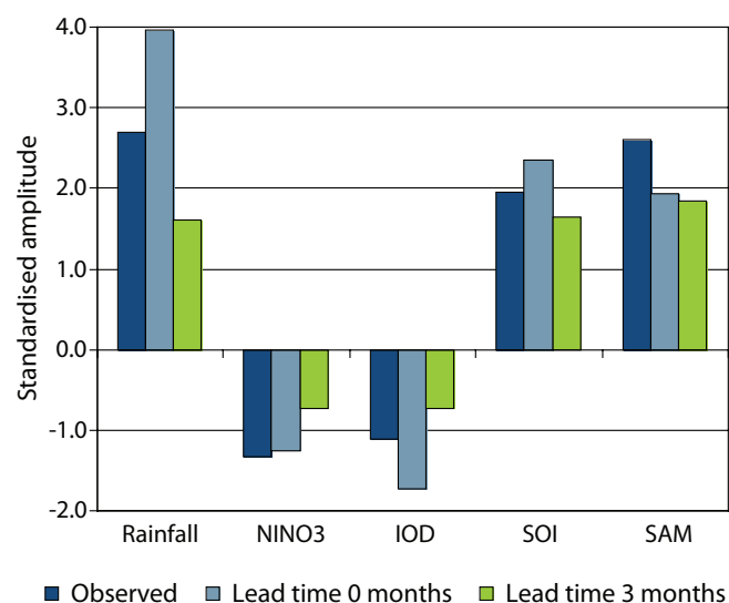
Figure 22. Observed and predicted (lead time 0 months in light blue, 3 months in green) anomalies of various climate indices for spring 2010. From left to right they are: rainfall averaged over south-eastern Australia (here defined as 25°–40° S, east of 135° E), and the NINO3, IOD, SOI and SAM indices. Magnitudes of the indices are in respective standard deviations.
