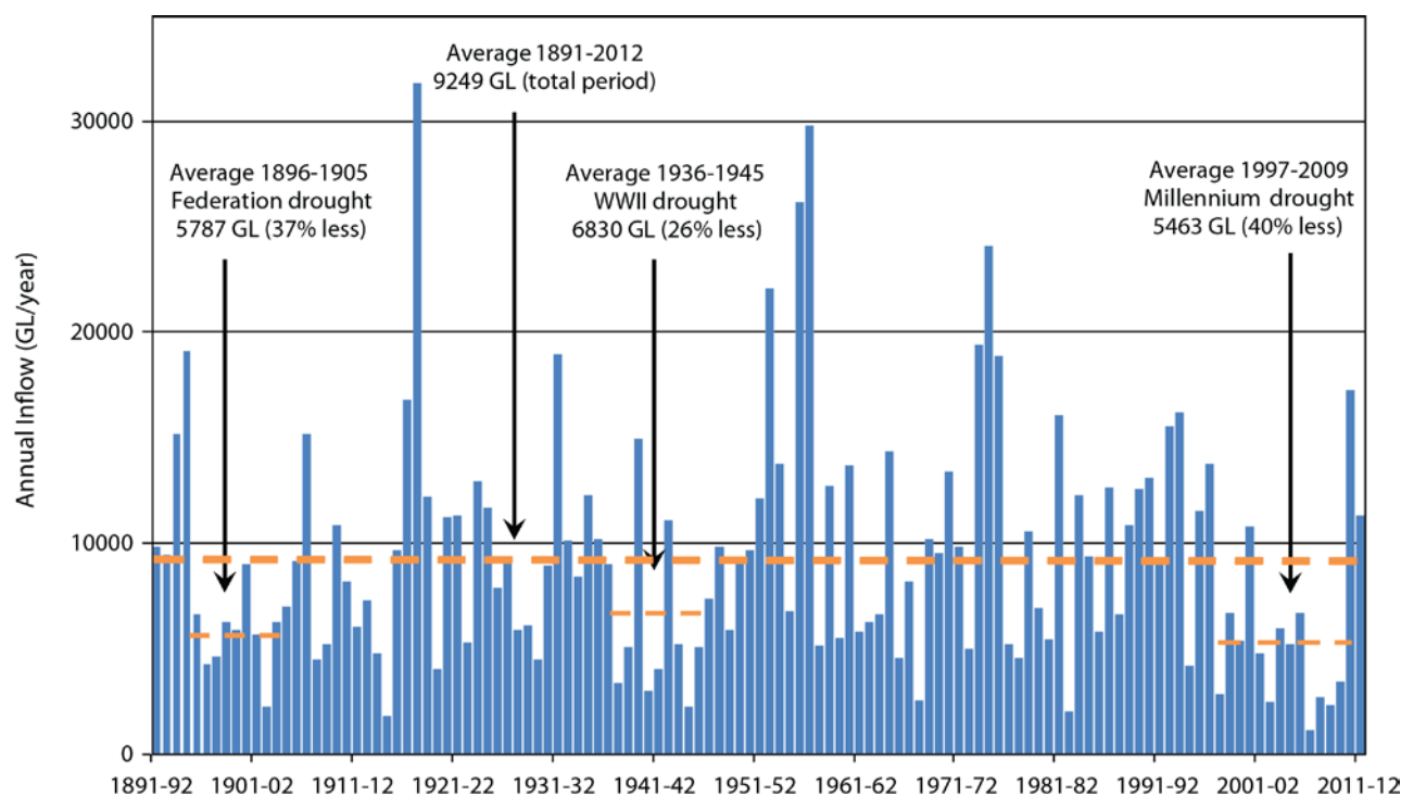
Figure 16. Annual total inflows into the River Murray showing the long-term average, and average inflows during the Millennium (1997-2009), World War II (1936-1945) and Federation (1896-1905) droughts.
