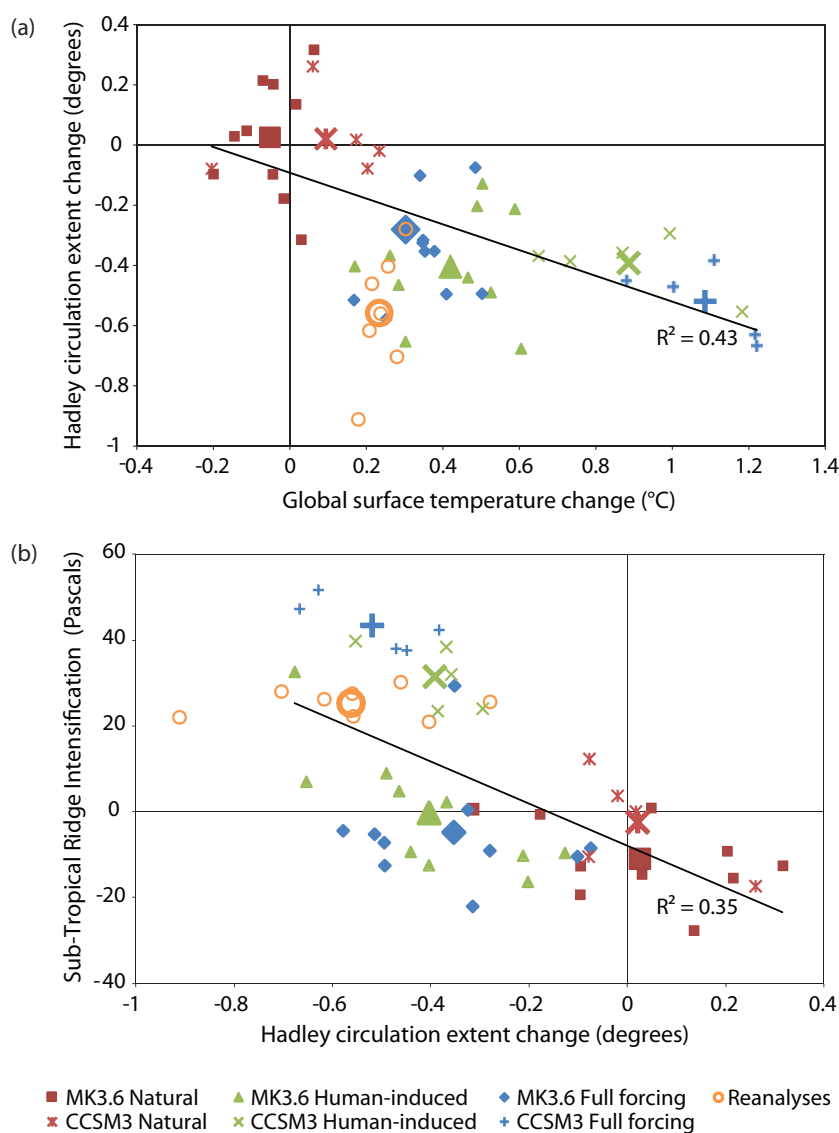
Figure 9. (a) Relationship between global warming and Hadley circulation expansion and (b) between Hadley circulation expansion and sub-tropical ridge intensification across a range of global datasets: eight reanalyses (orange circle), two climate model simulations (NCAR CCSM3 and CSIRO Mk 3.6) of the 20th century using different external inputs (natural only: red symbols, human-induced: green symbols and full forcing: blue symbols). In all instances, individual model simulations are shown as well as model averages (bold).
