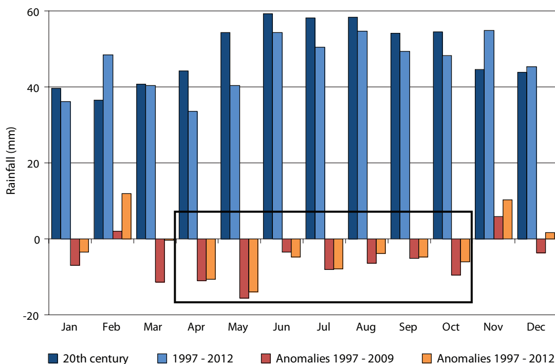
Figure 5. Monthly mean rainfall across south-eastern Australian for the 20th century (dark blue bars) and for the period January 1997 to July 2012 (light blue bars). Anomalies from the 20th century climatology during this latter period (1997–2012) are shown as orange bars and anomalies for the period of the Millennium drought (1997–2009) are shown as red bars. Cool season months with negative rainfall anomalies since 1997 (outlined with a black box) remained similar despite the addition of the very wet 2010–12 years, in contrast to the warm season months where the differences between the orange and red bars are much larger.
