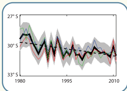
(a) Edge of the tropical tropopause is moving south
