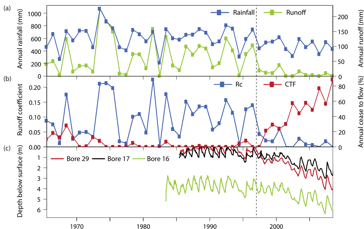
Figure 18. Annual time series of hydrologic metrics for the Axe Creek catchment in north-central Victoria. (a) shows rainfall (blue line) and runoff (green line); (b) shows the runoff coefficient, Rc (blue line) and cease to flow, CTF (red line); (c) shows groundwater levels for three different bores in the catchment.
