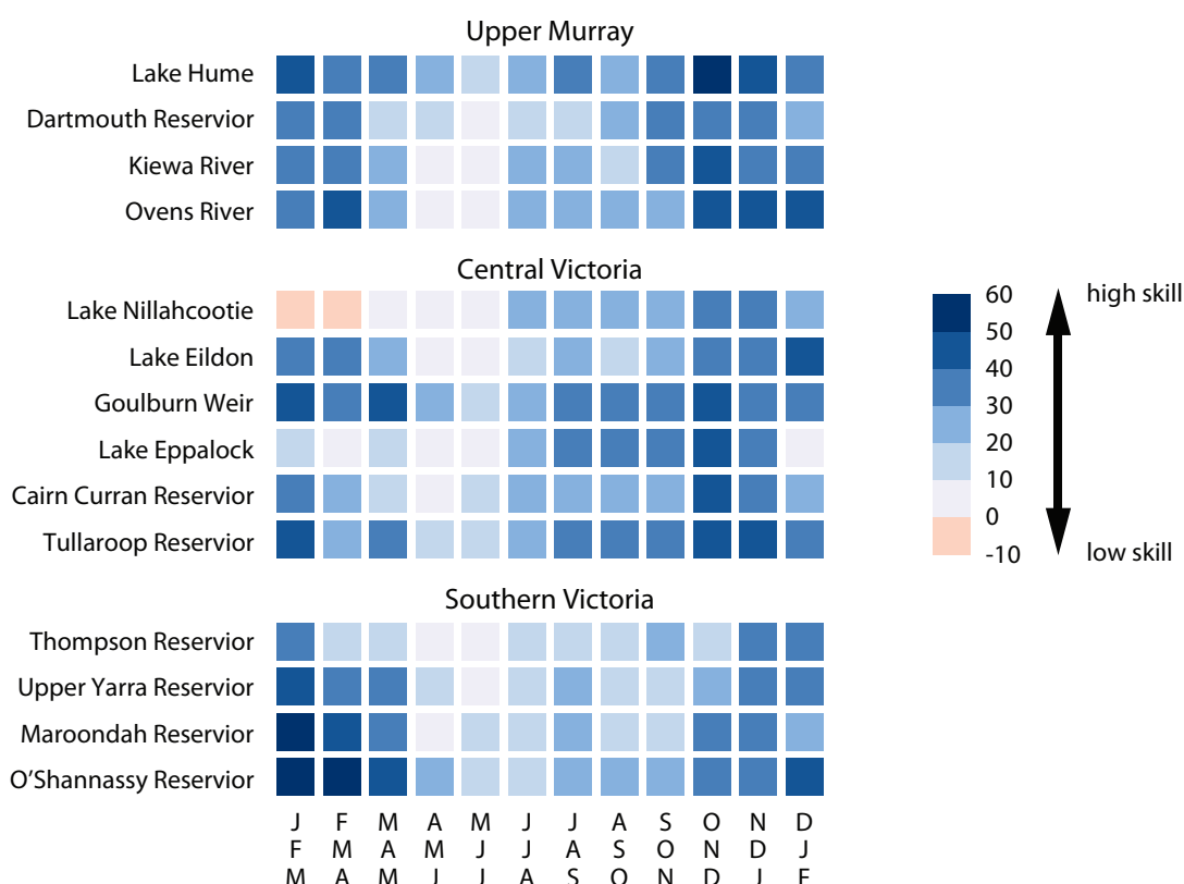
Figure 24. Skill score, in percentage and based on root mean squared error in probability, of merged seasonal streamflow forecasts for 12 overlapping seasons at 14 catchments.
