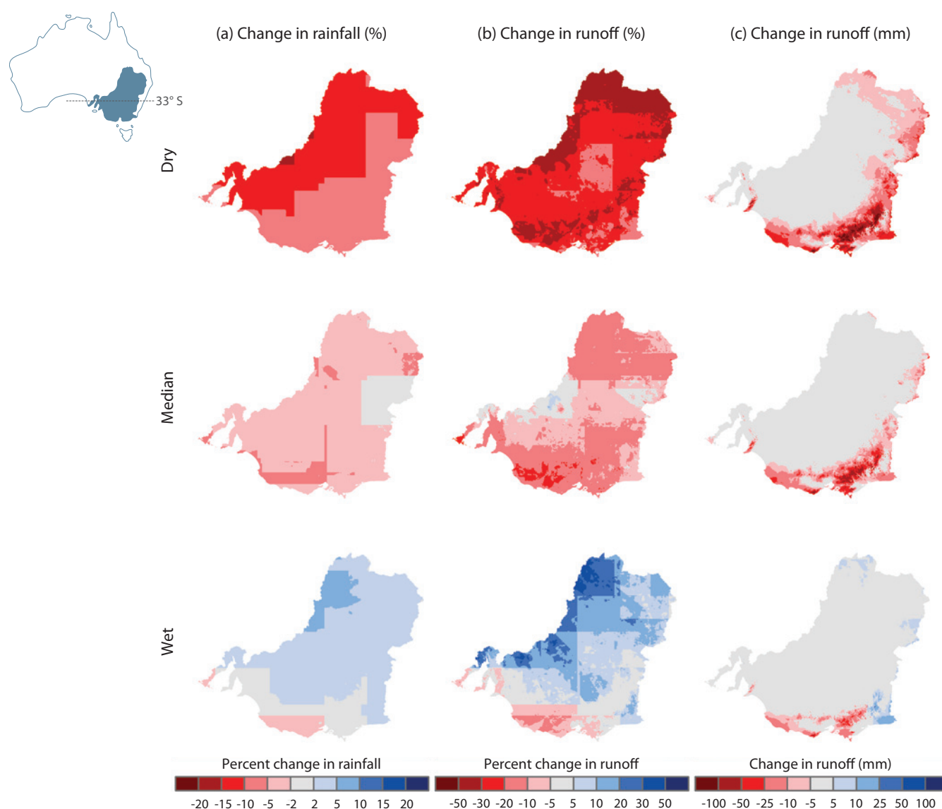
Figure 19. Projected change in (a) mean annual rainfall (percent change); (b) mean annual runoff (percent change); and (c) mean annual runoff (mm change) for a 1 °C global warming. The dry and wet estimates represent the 10th and 90th percentile of projected changes based on the outputs of 15 global climate models.
