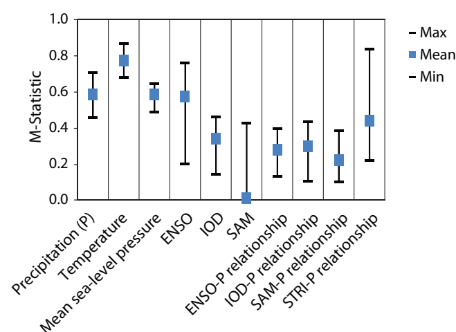
Figure 12. Range of M-Statistic summarising the ability of the 23 CMIP3 models to simulate the observed historical (1961–2000) characteristics over south-eastern Australia. An M-Statistic of 1 indicates a perfect match between the modelled and observed values and an M-Statistic of 0 indicates a very poor match.
