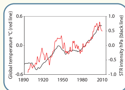
(d) Intensity of STR is related to global temperature
