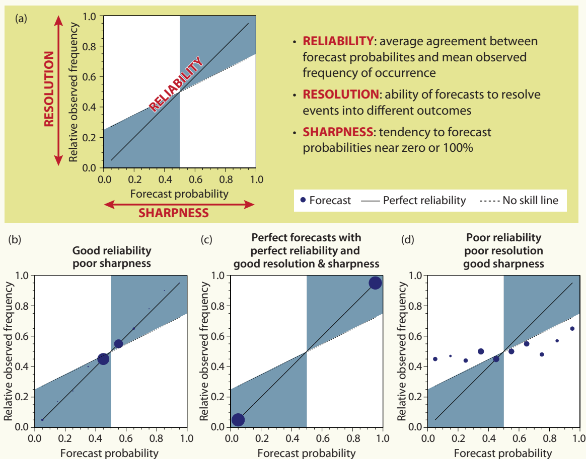
Figure 21. Example attributes diagrams demonstrating representation of reliability, resolution, and sharpness of forecasts (in this case, the probability of exceeding median rainfall).
