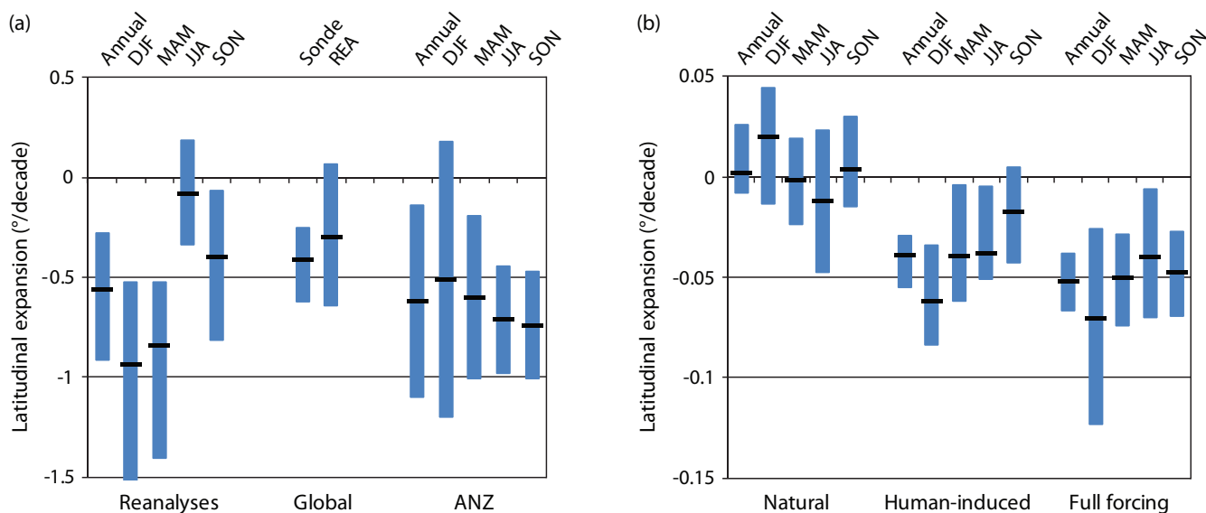
Figure 8. Trends in degrees latitude per decade for a range of indicators of the Hadley circulation expansion. (a) Average of Hadley circulation width from eight reanalysis datasets, edge of the tropics for the globe as derived from radiosonde data alone (Sonde) and from radiosonde and reanalyses data (REA) for the annual mean alone, and for just Australia and New Zealand (ANZ) for the annual mean and the four calendar seasons as derived from radiosonde data alone. (b) Expansion of the tropics as modelled by a global climate model (CCSM3), for natural forcing alone, human-induced forcing alone, and full forcing. Note the different scales on y-axes of the two figures. The black line represents the median and the blue bar the range of results.
