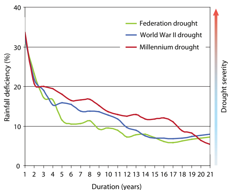
Figure 3. Drought depth duration curves computed using annual rainfall for periods from 1 to 21 years for three historical droughts: Federation drought in green, World War II drought in blue and Millennium drought in red. The severity of the drought increases up the graph with units on the y-axis showing the rainfall deficiency as a percent reduction compared to 1872–2009. The Millennium drought was the worst drought in the instrumental record for all durations between 3 and 19 years. (Source: Timbal and Fawcett, in press).
