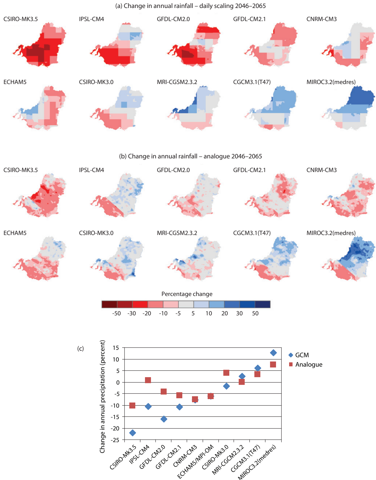
Figure 14. (a) Percentage change in future mean annual rainfall (2046–2065 relative to 1961–2000) across south-eastern Australia from (a) 10 global climate models; (b) analogue downscaling of the same models, and (c) percentage change averaged over the south-eastern Australian region.
