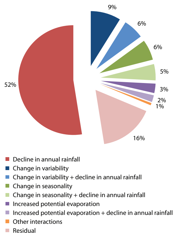
Figure 17. Relative climate influences on the observed decline in streamflow from the Campaspe River catchment in north-central Victoria during the Millennium drought. Change in variability refers to the lack of high rainfall events and change in seasonality refers to the larger decline in rainfall in the autumn and winter months.
