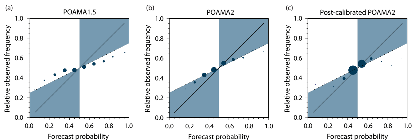
Figure 20. Accuracy and reliability of (a) POAMA1.5, (b) POAMA2 and (c) post-calibrated POAMA2 forecasts of above median rainfall for south-eastern Australia. Forecasts for all points across south-eastern Australia are used for all 12 seasons during 1980–2006 at lead time one month. The size of dots represents forecast frequency in each forecast category. Forecasts in the blue areas are considered to be skilful as they are correct in predicting the occurrence/non-occurrence of above median rainfall, and their errors are smaller than a climatological forecast.
