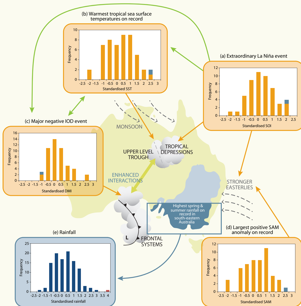
Figure 7. Indices of the internal modes of climate variability relevant to the 2010-11 floods in south-eastern Australia. Histograms for spring season (a) Southern Oscillation Index (SOI); (b) Sea-surface temperatures (SST) north of Australia; (c) Indian Ocean Dipole (as measured by the Dipole Mode Index, DMI) and (d) Southern Annular Mode (SAM) show that the 2010 anomalies (indicated by light blue bars) were at the most extreme end of their distributions for the past 51 years. As a result, spring-summer rainfall in 2010/11 (e) was the highest on record (shown in red). The elements shown on the map of Australia are the meteorological elements through which the identified modes of climate variability influence the rainfall of south-eastern Australia (as shown by the orange arrows). Green arrows indicate interactions between the climatic elements.
