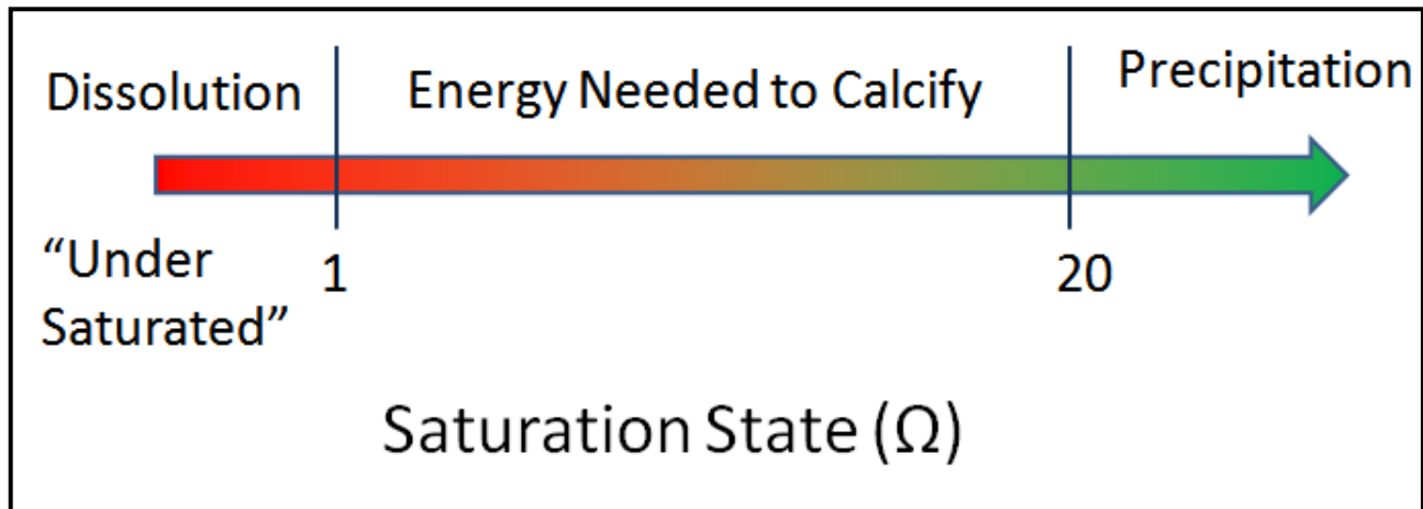
Figure 3.2.12. Relationship between saturation state and the formation of calcium carbonate in seawater.
