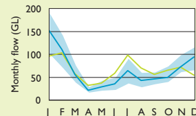
6. Gwydir at Gravesend Road Bridge
