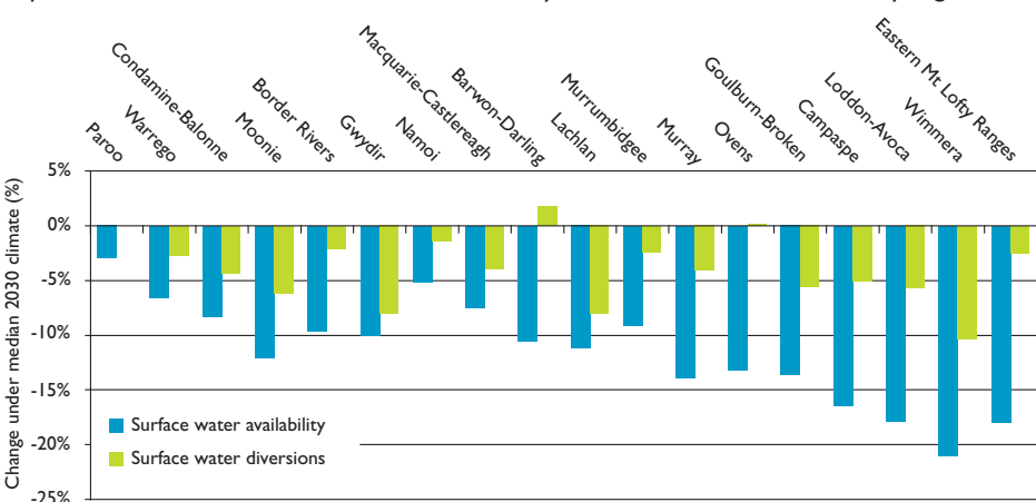
Impact of median 2030 climate on water availability and surface water diversions by region
