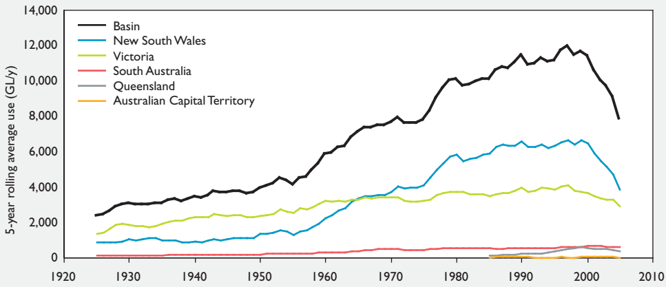
Growth in total and jurisdictional surface water use in the MDB (five-year moving averages)
