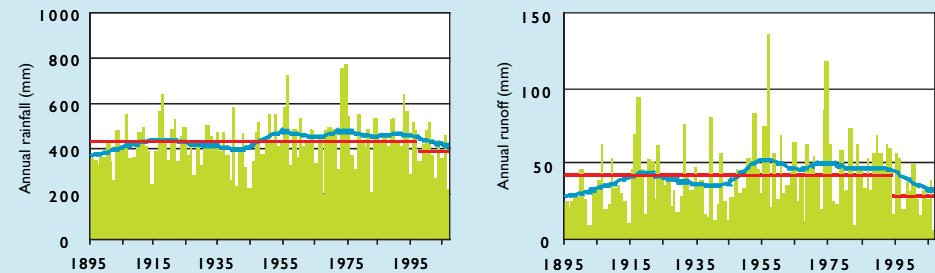
Annual rainfall (left) and modelled annual runoff (right) averaged over the southern MDB (Murrumbidgee, Murray, Ovens, Goulburn-Broken, Campaspe, Loddon-Avoca, Wimmera and Eastern Mount Lofty Ranges regions). Smoothed lines indicate longer term variability. Red lines indicate the 1895–1996 and 1997–2006 average values
