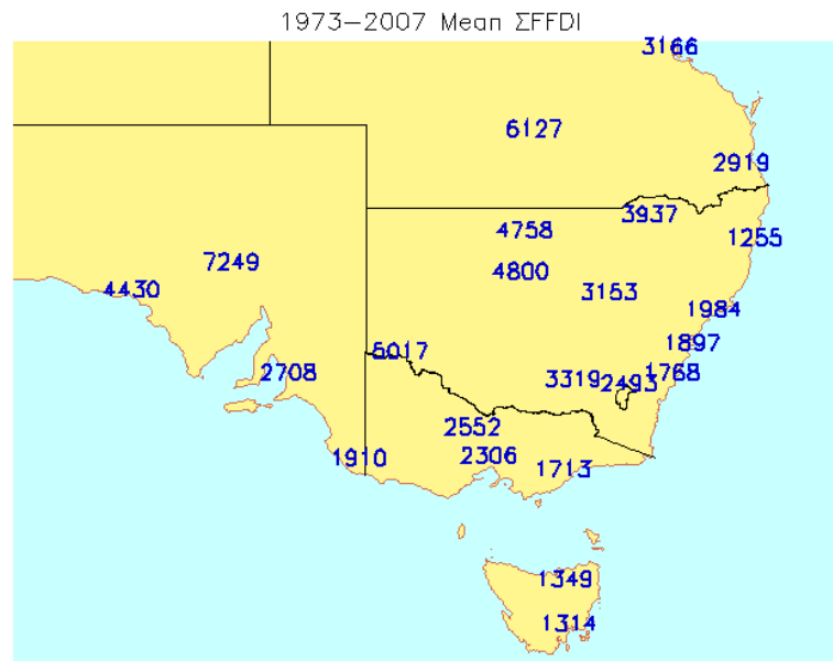
Figure 17. Average annual \Sigma FFDI for the 1973-74 through 2006-07 fire seasons. Brisbane, Laverton and Richmond are not shown for clarity.
