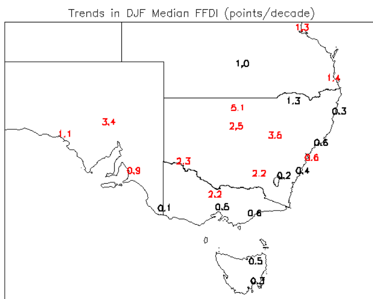
Figure 25. Map of observed trends in summer (DJF) median FFDI. Units are points per decade. Red numbers are significant at the 95% level.
