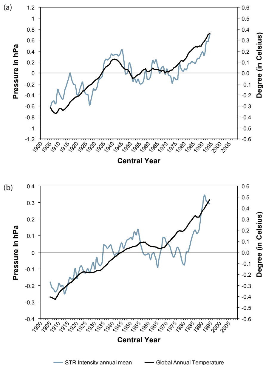
Figure 5. Time series of anomalies of annual STR intensity (in hPa on the left Y-axis) and global temperature (in °C on the right Y-axis) calculated from (a) observations, and (b) the average number of simulations with a state-of-the-art climate model forced with a combination of processes (Timbal et al., 2009).
