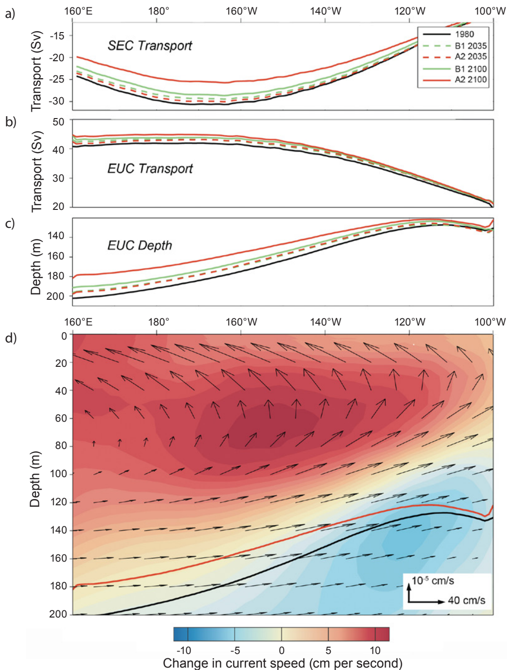
Figure 3.27 Projected changes in (a) transport volume ( Sv = 10^6 \text{ m}^3 \text{ per second} ) of the South Equatorial Current (SEC) as a function of longitude across the equator; (b) transport volume of the Equatorial Undercurrent (EUC); (c) depth of the EUC; and (d) eastward velocity (cm per second) for the A2 scenario in 2100 (2080–2099) minus (1980–1999), with mean velocity vectors superimposed as arrows (averaged between 2°S and 2°N with vertical velocity scale accentuated). Black and red lines indicate the mean position of the EUC core for 1980–1999, and for the A2 scenario in 2100, respectively.
