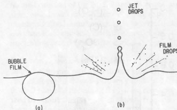
Figure 1. (a) An air bubble at an air-water interface. (b) The production of jet and film drops from a bursting air bubble. After Blanchard (1983).
