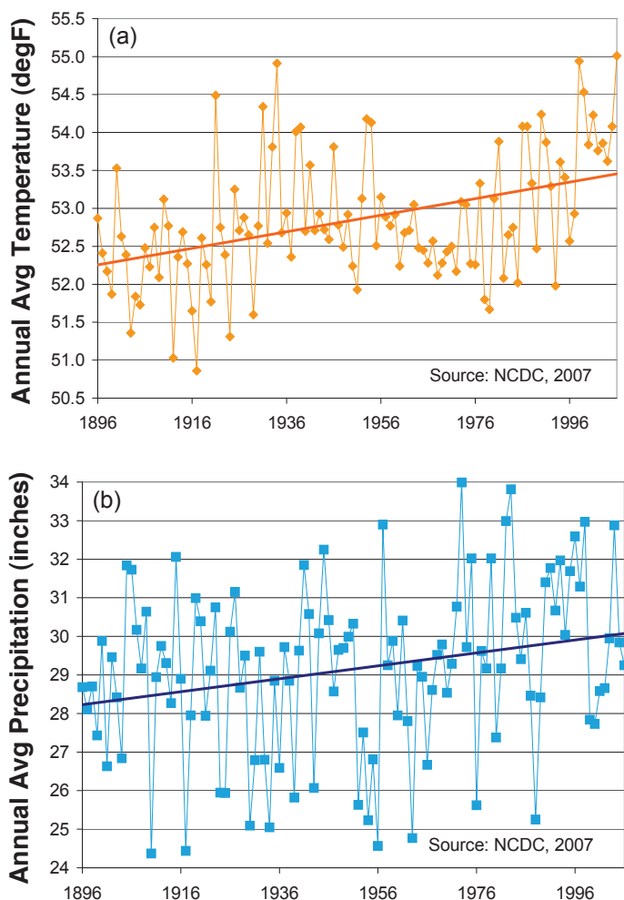
Figure 1.1 Observed trends in annual average (a) temperature (°F) and (b) precipitation (inches) across the continental United States from 1896 to 2006 (Source: NCDC, 2007)
