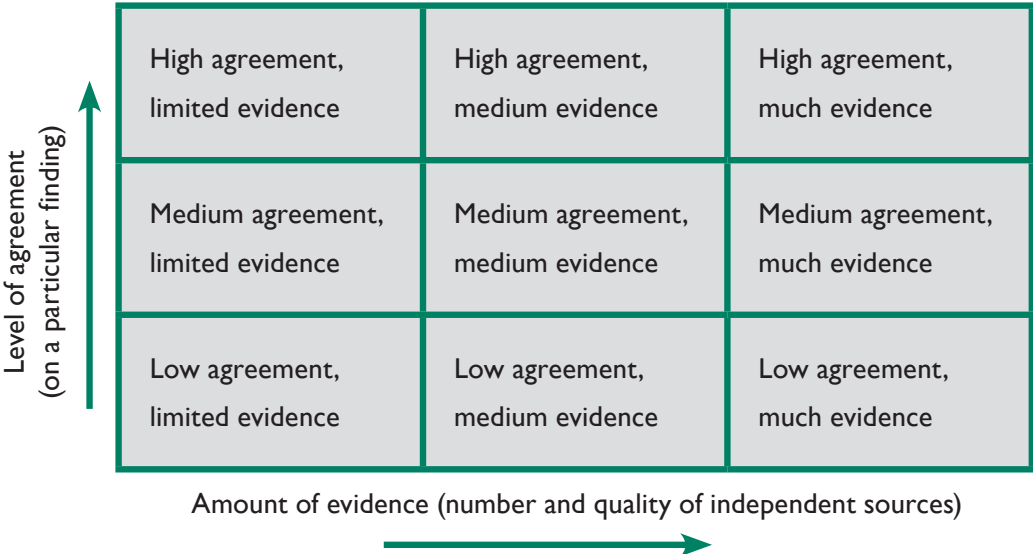
Figure I.5 Considerations in determining confidence Source: IPCC Guidance Notes on risk and uncertainty (2005)
