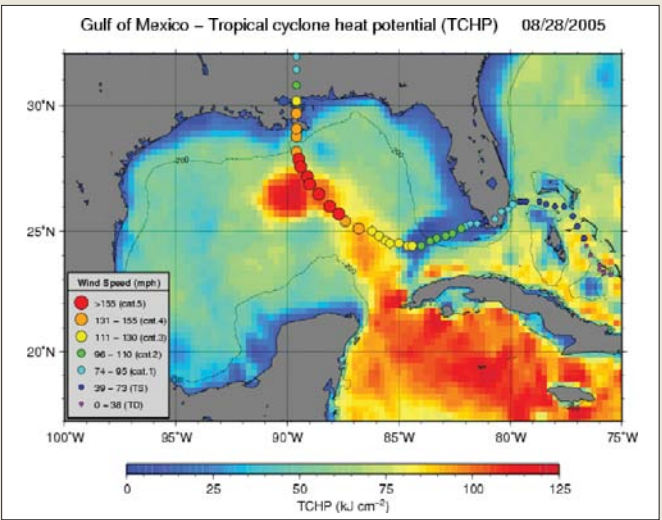
Tropical Cyclone Heat Potential associated with Hurricanes Katrina and Rita; the hurricanes grow in intensity as they pass over warm water
