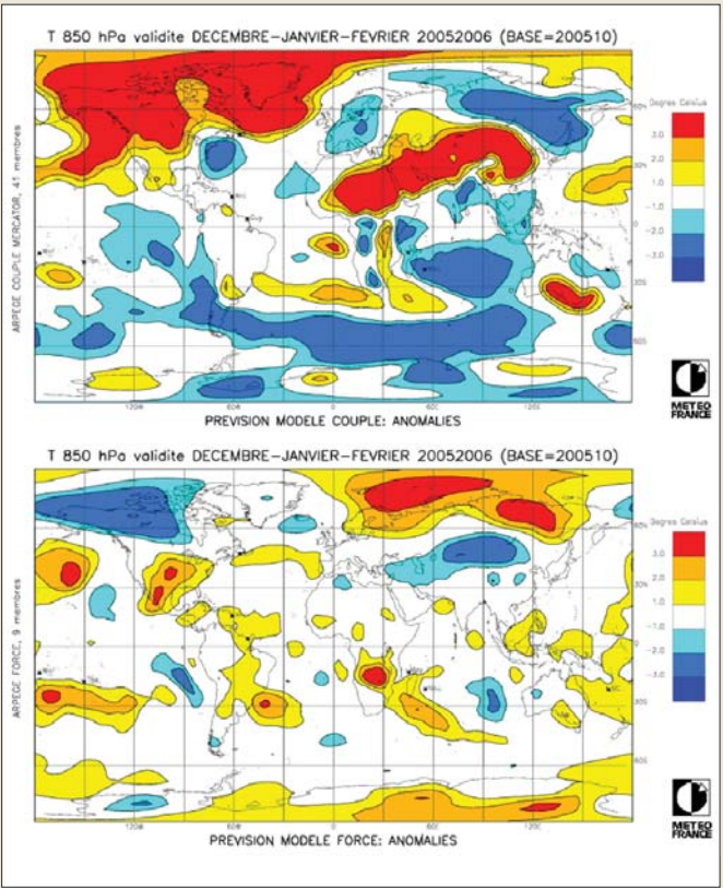
Composite figure showing the winter forecast for 2005-2006 with a coupled ocean atmosphere model initialized with (upper) and without (lower) the Mercator ocean analyses; the cold anomaly over Europe is missed without the ocean information
