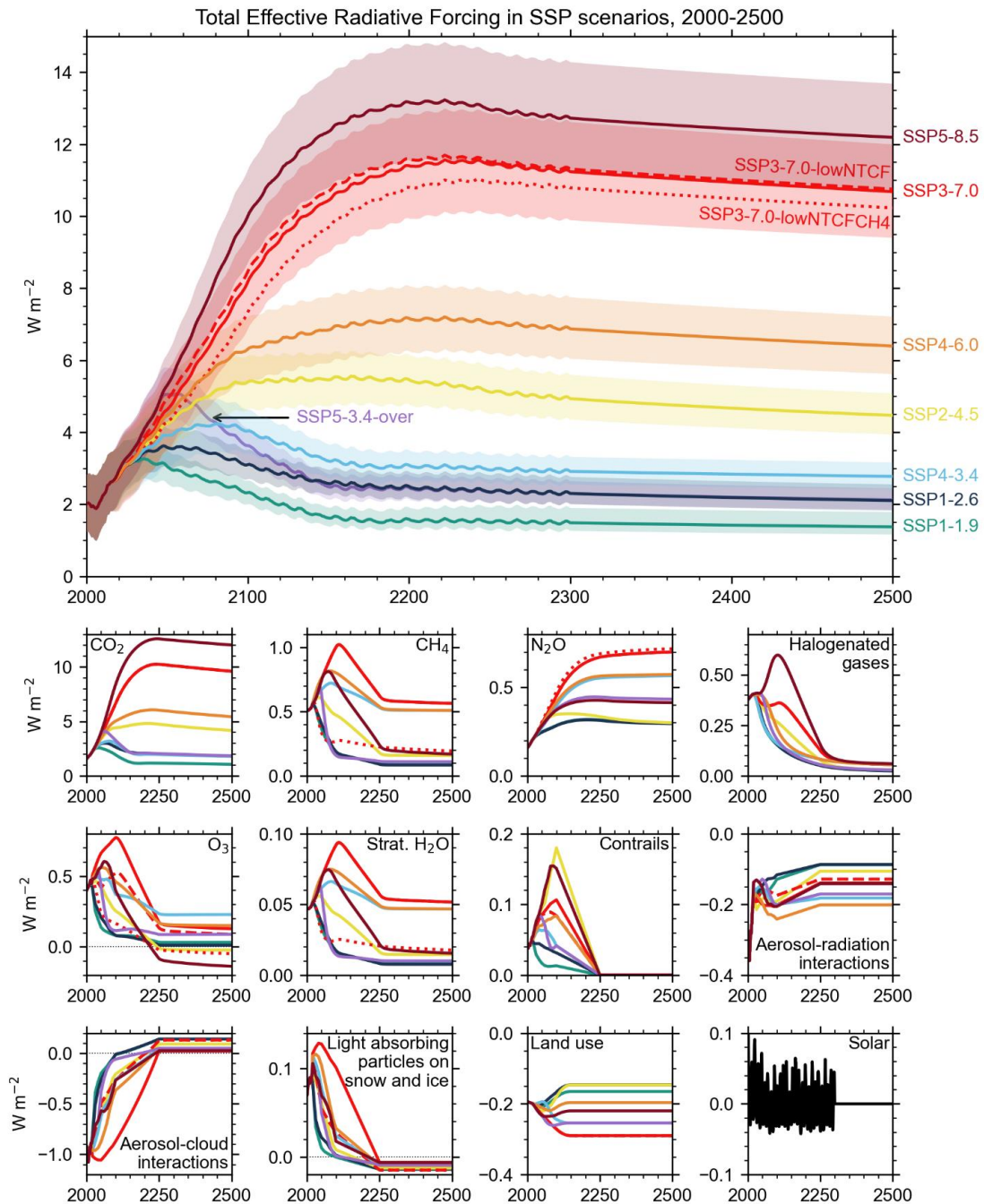
12 13 Figure 7.SM.1: Total effective radiative forcing from SSP scenarios with respect to 1750 for 2000-2500 (top panel), 14 showing best estimate and 5–95% uncertainty range (shaded regions). Uncertainty ranges are not 15 shown for SSP3-7.0-lowNTCF and SSP3-7.0-NTCFCH4 for visual clarity. Bottom matrix shows the
