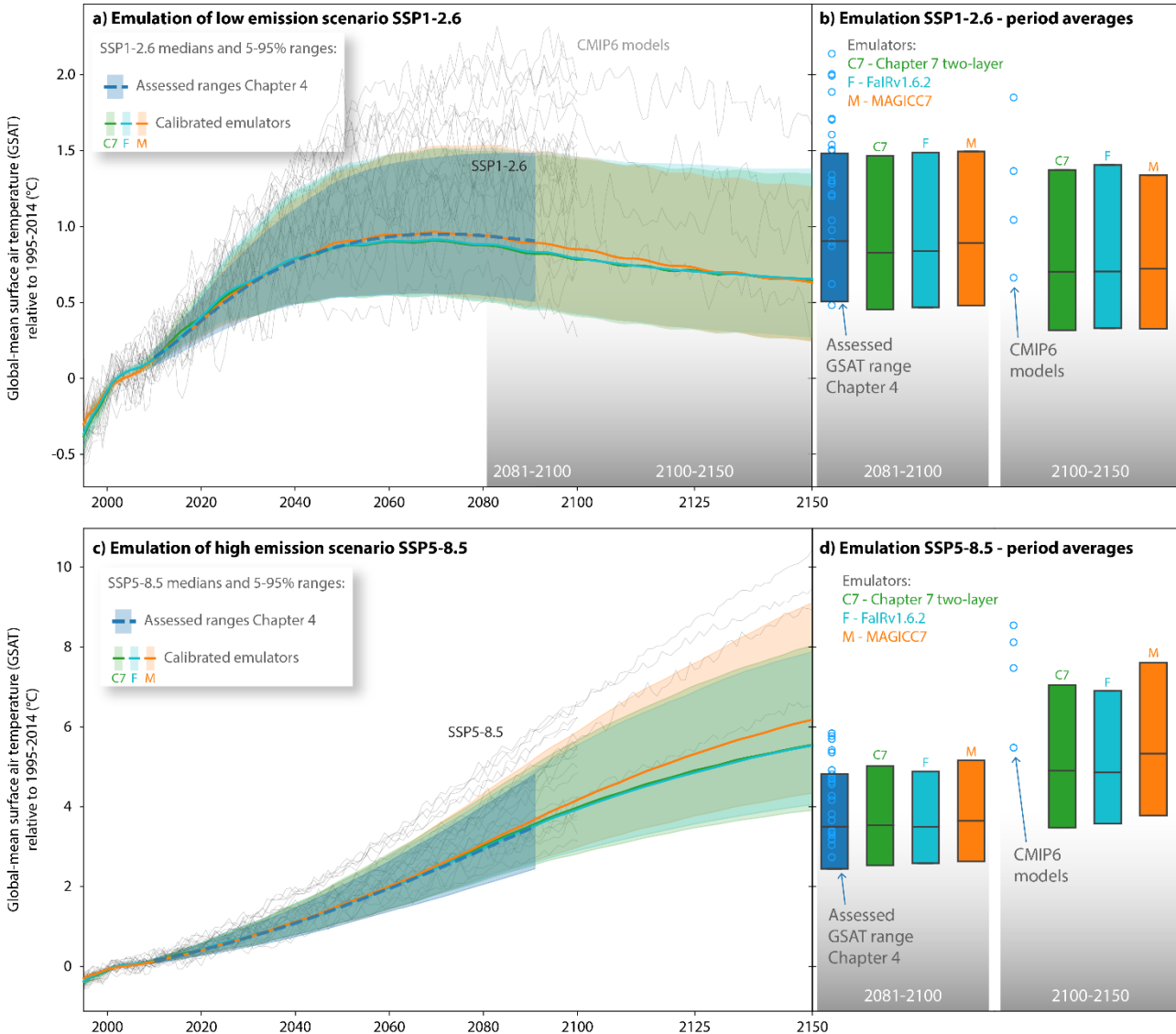
9 10 Figure 7.SM.2: (a) Time series and (b) 2100-2150 means of emulated GSAT projections from the Chapter 7 two-layer 11 model (green), FAIRv1.6.2 (light blue), and MAGICC7.5.1 (orange) from 1995 to 2150, following the 12 SSP1-2.6 scenario ((a) and (b)) and the SSP5-8.5 scenario ((c) and (d)). In (a) and (c) the ensemble 13 median estimates are solid lines and the 5–95% ranges are shaded; in (b) and (d) the bar range shows 14 5–95% ranges with the median in black. Overlaid CMIP6 model results are shown as lines in (a) and 15 (c), and dots in (b) and (d) (fewer dots are shown for the 2100–2150 period because only a limited 16 number of CMIP6 models have performed runs beyond 2100). In (a) and (c), Chapter 4 assessed 17 GSAT projections (20-year running means) are shown with a dark blue dashed line and 5-95% range 18 in dark blue shading. 19 20
