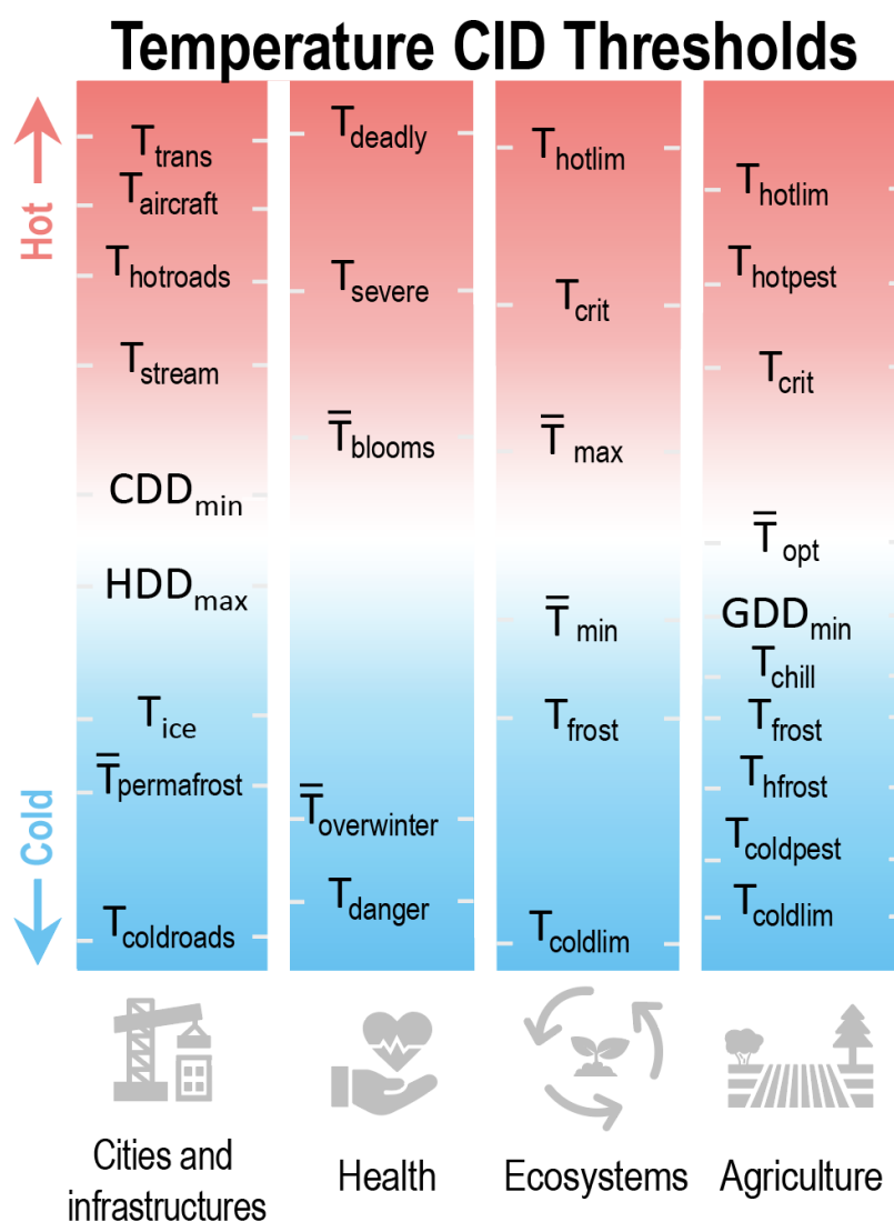
Figure 12.3: Conceptual illustration of representative climatic impact-driver thresholds showing how graduating thresholds affect successive sectoral assets and lead to potentially more acute hazards as conditions become more extreme (exact values are not shown as these must be tailored to reflect diverse vulnerabilities of regional assets). Representative threshold definitions ( T = instantaneous temperature; \bar{T} = mean temperature): Cities and Infrastructures : T_{trans} = temperature at which energy transmission lines efficiency reduced; T_{aircraft} = temperature at which aircraft become weight-restricted for takeoff; T_{hotroads} = temperature above which roads begin to warp; T_{stream} = temperature at which streams are not capable of adequately cooling thermal plants; CDD_{min} = Minimum temperature for calculating cooling degree days; HDD_{min} = maximum temperature for calculating heating degree days; T_{ice} = temperature at which ice threatens transportation; \bar{T}_{permafrost} = mean seasonal temperature above which permafrost thaws at critical depths; T_{coldroads} = temperature below which road asphalt performance suffers. Health : T_{deadly} = temperatures above which prolonged exposure may be deadly (often combined with humidity for heat indices); T_{severe} = temperatures above which prolonged exposure may cause elevated morbidity; \bar{T}_{blooms} = mean temperature for harmful algal or cyanobacteria blooms; T_{danger} = level of dangerous cold temperatures (often combined with wind for chill indices); T_{overwinter} = temperature below which disease vector species cannot survive winter. Ecosystems (CID indices for air and ocean temperature): T_{hotlim} and T_{coldlim} = limiting hot and cold temperatures for a given species range; T_{frost} = frost threshold; \bar{T}_{max} and \bar{T}_{min} = maximum and minimum suitable annual mean temperatures for a given species; T_{crit} = critical temperature above which a given species is stressed. Agriculture : T_{hotlim} = temperature above which a crop or livestock species dies; T_{hotpest} = maximum (or ‘lethal’) temperature above which an agricultural pest/disease/weed cannot survive; T_{crit} = temperature at which productivity for a given crop is depressed; \bar{T}_{opt} = optimal mean temperature for a given plant’s productivity; GDD_{min} = threshold temperature for growing degree days determining plant development; T_{chill} = temperature below which chilling units are accumulated; T_{frost} = temperature below which frost occurs; T_{hfrost} = temperature
