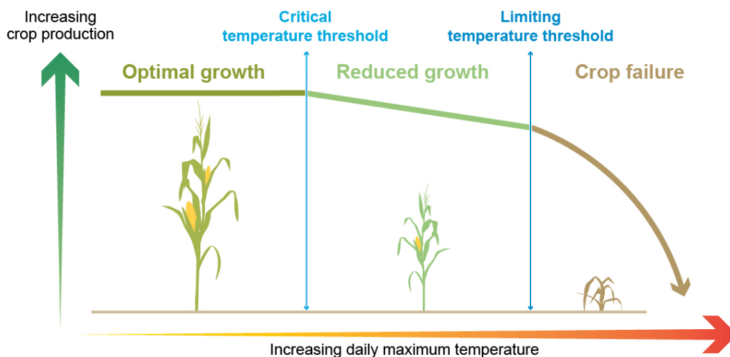
FAQ12.2, Figure 1: Crop response to maximum temperature thresholds. Crop growth rate responds to daily maximum temperature increases, leading to reduced growth and crop failure as temperatures exceed critical and limiting temperature thresholds, respectively. Note that changes in other environmental factors (such as carbon dioxide and water) may increase the tolerance of plants to increasing temperatures.
