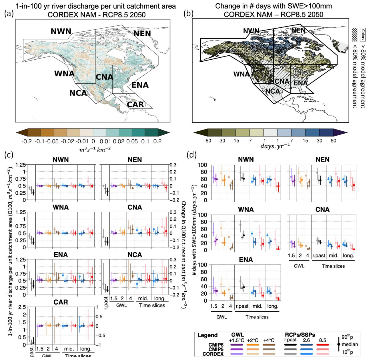
Figure 12.10: Projected changes in selected climatic impact-driver indices for North America. (a) Mean change in 1-in-100 year river discharge per unit catchment area ( Q100, m^3 s^{-1} km^{-2} ), and (b) median change in the number of days with snow water equivalent (SWE) over 100 mm (from November to March), from CORDEX-North America models for 2041-2060 relative to 1995-2014 and RCP8.5. Diagonal lines indicate where less than 80% of models agree on the sign of change. (c) Bar plots for Q100 (m^3 s^{-1} km^{-2}) averaged over land areas for the WGI reference AR6 regions (defined in Chapter 1). The left column within each panel (associated with the left y-axis) shows the 'recent past' (1995-2014) Q100 absolute values in grey shades. The other columns (associated with the right y-axis) show the Q100 changes relative to the recent past values for two time periods ('mid' 2041-2060 and 'long' 2081-2100) and for three global warming levels (defined relative to the preindustrial period 1850-1900): 1.5°C (purple), 2°C (yellow) and 4°C (brown). The bars show the median (dots) and the 10 th -90 th percentile range of model ensemble values across each model ensemble. CMIP6 is shown by the darkest colours, CMIP5 by medium, and CORDEX by light. SSP5-8.5/RCP8.5 is shown in red and SSP1-2.6/RCP2.6 in blue. (d) As for (c) but showing absolute values for number of days with SWE > 100mm, masked to grid cells with at least 14 such days in the recent-past. See Technical Annex VI for details of indices. A Caribbean Q100 bar plot is included here but assessed in the Small islands section (12.4.7). Further details on data sources and processing are available in the chapter data table (Table 12.SM.1).
