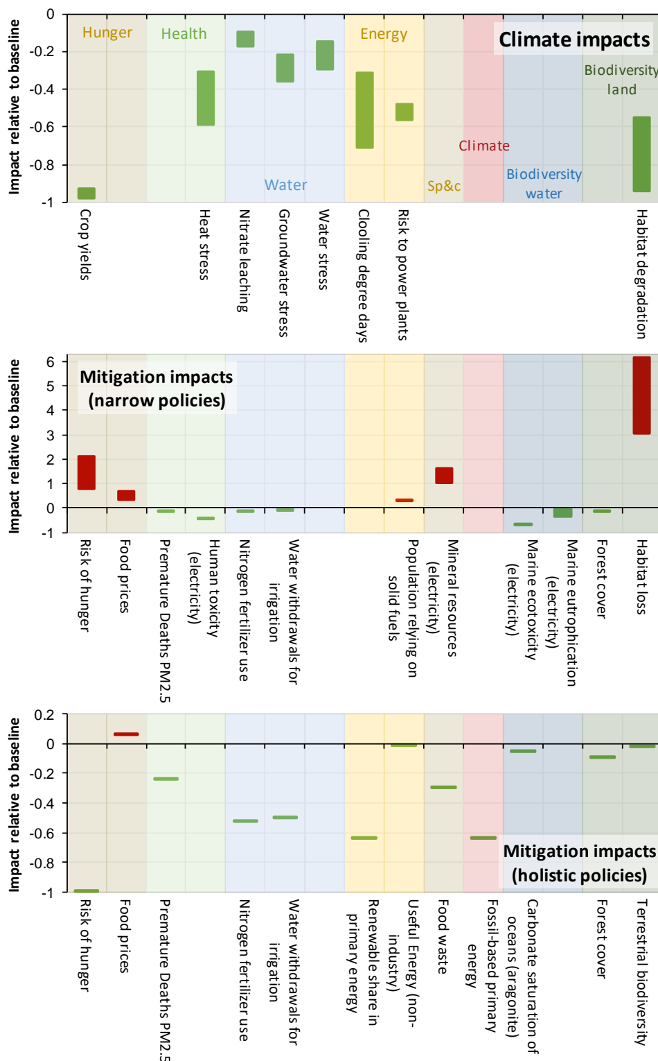
Figure 3.41: Adverse (>0) and beneficial (<0) consequences of mitigation for 1.5°C compared to national policy, due to climate impacts (top; Byers et al. (2018)), narrowly focused mitigation actions (middle; Krey et al (2019b), submitted) and holistic mitigation actions focused upon avoiding trade-offs (bottom; (Soergel et al. 2021))
