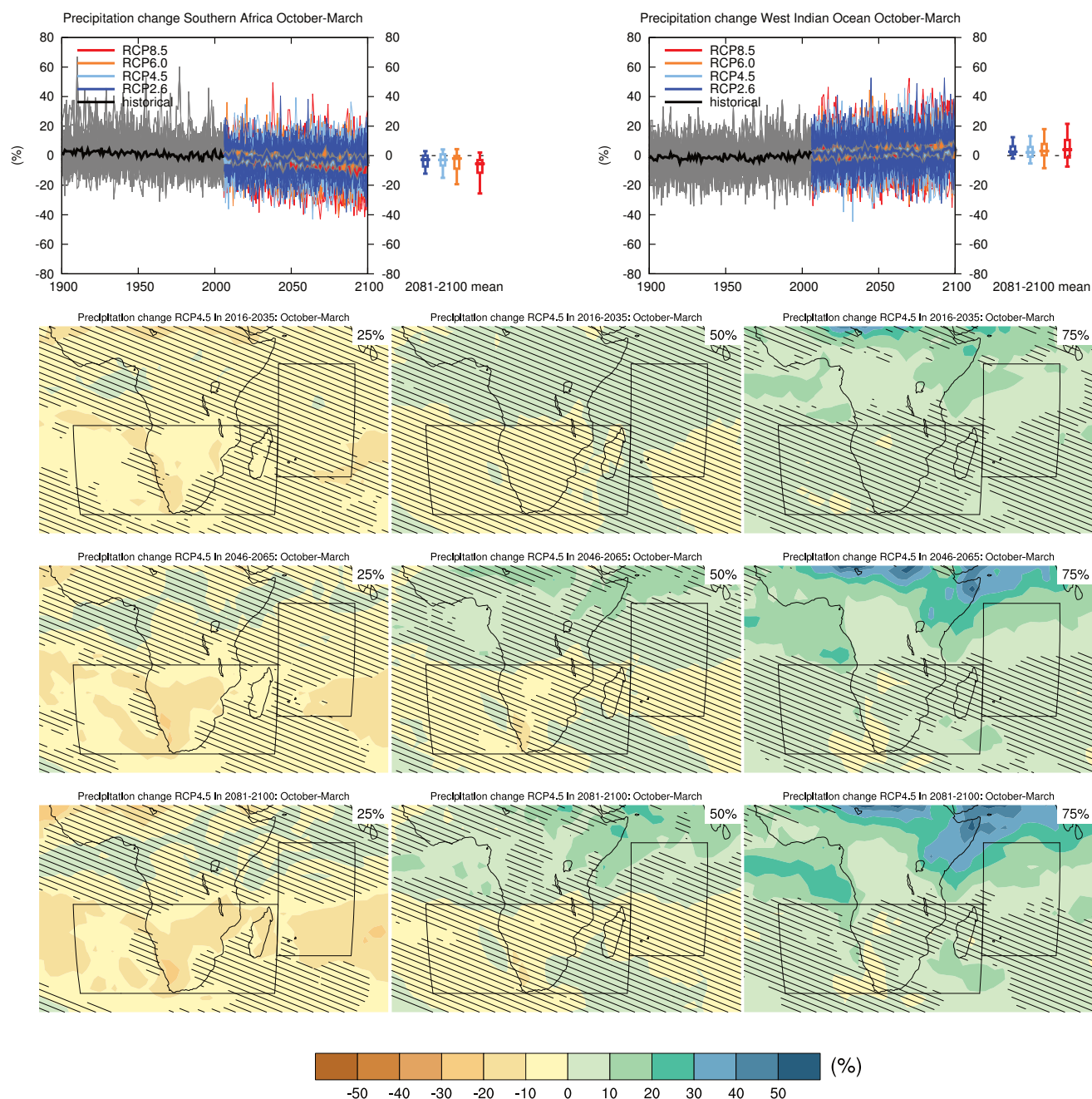
Figure AI.SM4.5.98 | (Top left) Time series of relative change relative to 1986–2005 in precipitation averaged over land grid points in Southern Africa (35°S to 11.4°S, 10°W to 52°E) in October to March. (Top right) Same for sea grid points in the West Indian Ocean (25°S to 5°N, 52°E to 75°E). Thin lines denote one ensemble member per model, thick lines the CMIP5 multi-model mean. On the right-hand side the 5th, 25th, 50th (median), 75th and 95th percentiles of the distribution of 20-year mean changes are given for 2081–2100 in the four RCP scenarios.
