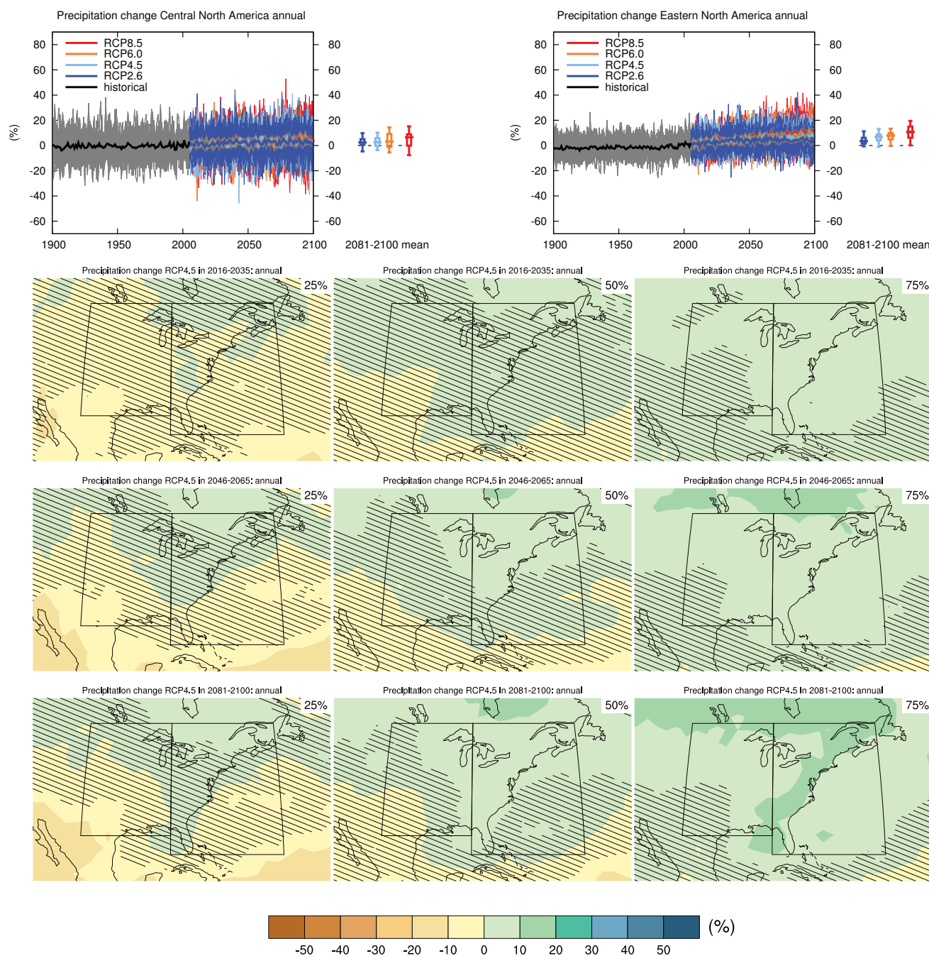
Figure AI.SM4.5.41 | (Top left) Time series of relative change relative to 1986–2005 in annual precipitation averaged over land grid points in Central North America (28.6°N to 50°N, 105°W to 85°W). (Top right) Same for land grid points in Eastern North America (25°N to 50°N, 85°W to 60°W). Thin lines denote one ensemble member per model, thick lines the CMIP5 multi-model mean. On the right-hand side the 5th, 25th, 50th (median), 75th and 95th percentiles of the distribution of 20-year mean changes are given for 2081–2100 in the four RCP scenarios.
