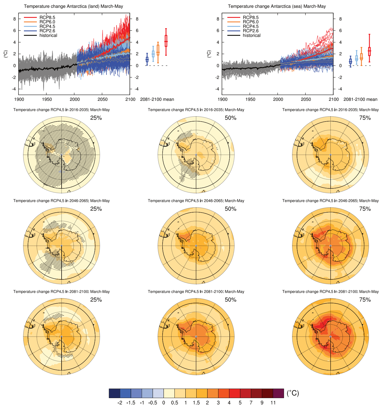
Figure AI.SM4.5.150 | (Top left) Time series of temperature change relative to 1986–2005 averaged over land grid points in Antarctica (90°S to 50°S) in March to May. (Top right) Same for sea grid points. Thin lines denote one ensemble member per model, thick lines the CMIP5 multi-model mean. On the right-hand side the 5th, 25th, 50th (median), 75th and 95th percentiles of the distribution of 20-year mean changes are given for 2081–2100 in the four RCP scenarios.
