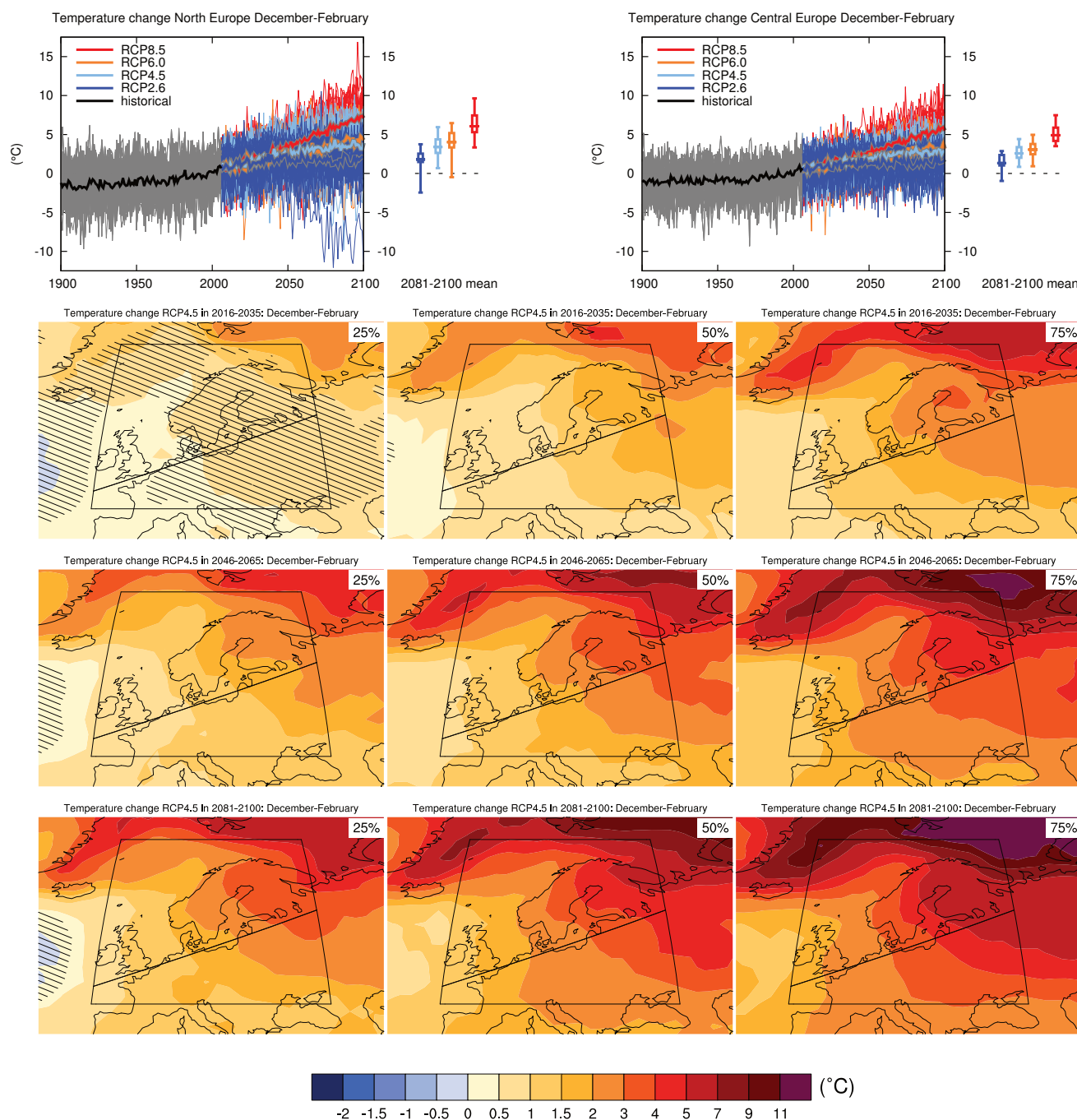
Figure AI.SM4.5.69 | (Top left) Time series of temperature change relative to 1986–2005 averaged over land grid points in North Europe (10°W, 48°N; 10°W, 75°N; 40°E, 75°N; 40°E, 61.3°N) in December to February. (Top right) Same for land grid points in Central Europe (10°W, 45°N; 10°W, 48°N; 40°E, 61.3°N; 40°E, 45°N). Thin lines denote one ensemble member per model, thick lines the CMIP5 multi-model mean. On the right-hand side the 5th, 25th, 50th (median), 75th and 95th percentiles of the distribution of 20-year mean changes are given for 2081–2100 in the four RCP scenarios.
