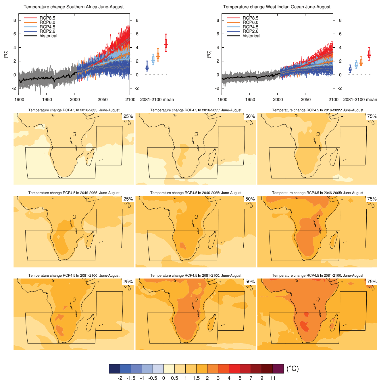
Figure AI.SM4.5.95 | (Top left) Time series of temperature change relative to 1986–2005 averaged over land grid points in Southern Africa (35°S to 11.4°S, 10°W to 52°E) in June to August. (Top right) Same for sea grid points in the West Indian Ocean (25°S to 5°N, 52°E to 75°E). Thin lines denote one ensemble member per model, thick lines the CMIP5 multi-model mean. On the right-hand side the 5th, 25th, 50th (median), 75th and 95th percentiles of the distribution of 20-year mean changes are given for 2081–2100 in the four RCP scenarios.
