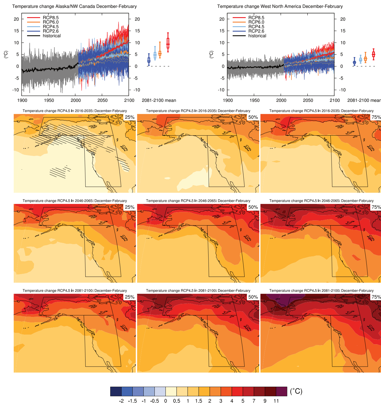
Figure AI.SM4.5.29 | (Top left) Time series of temperature change relative to 1986–2005 averaged over land grid points in Alaska/NW Canada (60°N to 72.6°N, 168°W to 105°W) in December to February. (Top right) Same for land grid points in West North America (28.6°N to 60°N, 130°W to 105°W). Thin lines denote one ensemble member per model, thick lines the CMIP5 multi-model mean. On the right-hand side the 5th, 25th, 50th (median), 75th and 95th percentiles of the distribution of 20-year mean changes are given for 2081–2100 in the four RCP scenarios.
