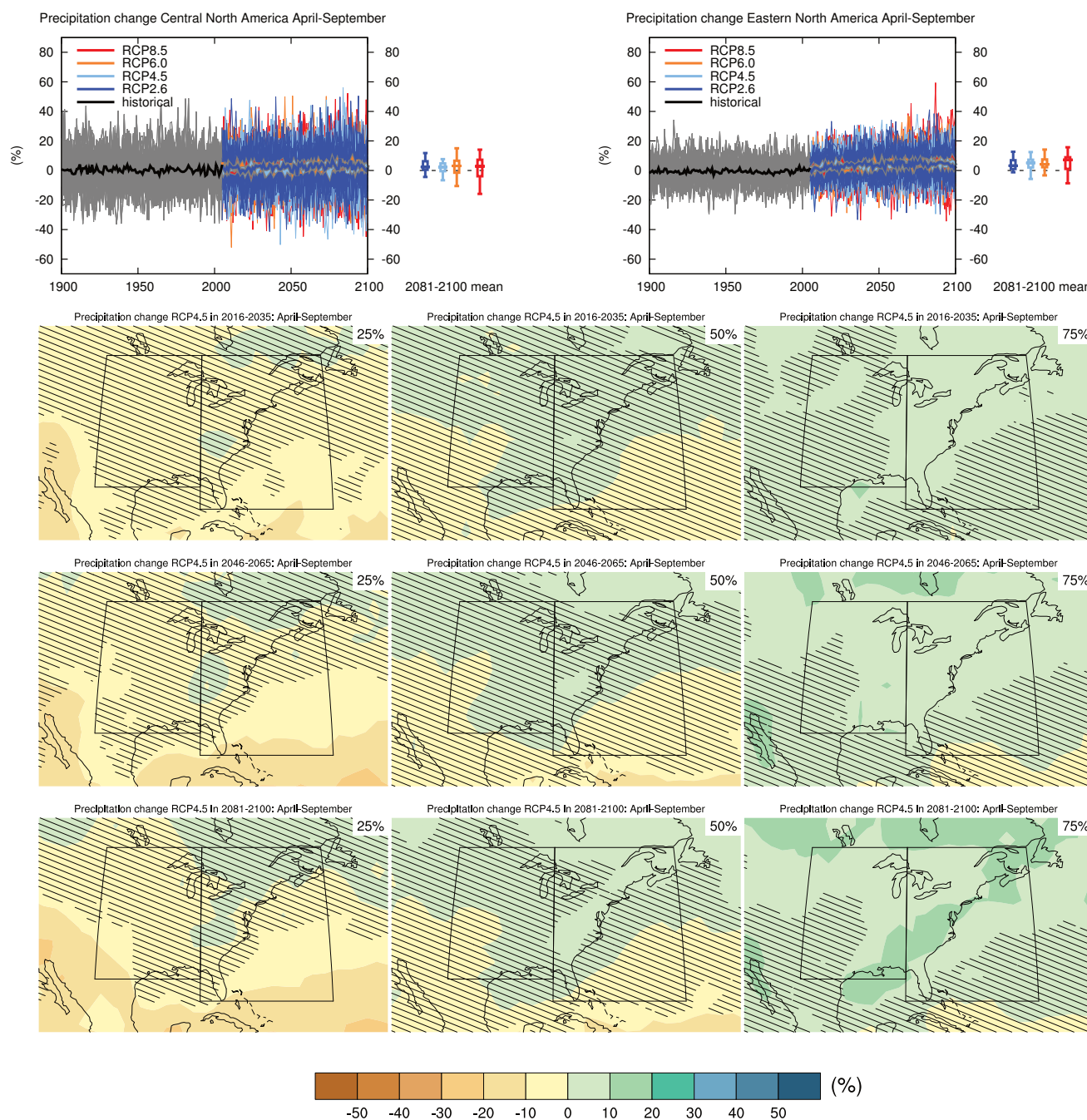
Figure AI.SM4.5.43 | (Top left) Time series of relative change relative to 1986–2005 in precipitation averaged over land grid points in Central North America (28.6°N to 50°N, 105°W to 85°W) in April to September. (Top right) Same for land grid points in Eastern North America (25°N to 50°N, 85°W to 60°W). Thin lines denote one ensemble member per model, thick lines the CMIP5 multi-model mean. On the right-hand side the 5th, 25th, 50th (median), 75th and 95th percentiles of the distribution of 20-year mean changes are given for 2081–2100 in the four RCP scenarios.
