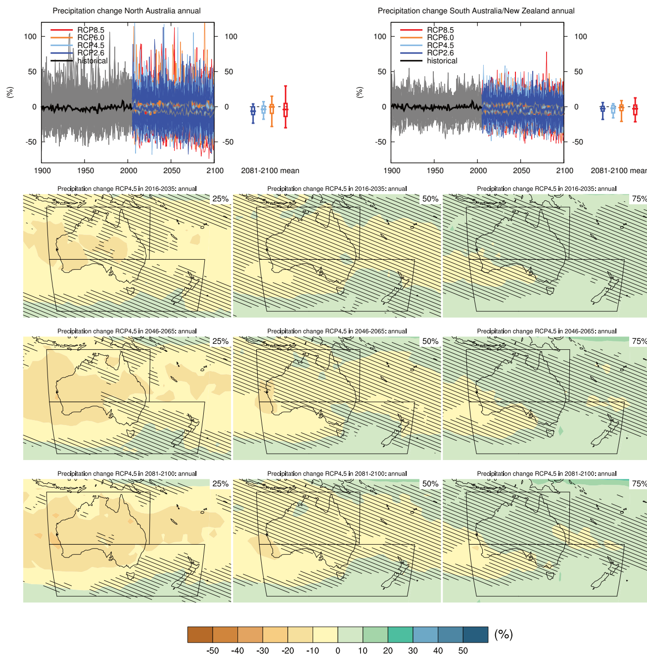
Figure AI.SM4.5.137 | (Top left) Time series of relative change relative to 1986–2005 in annual precipitation averaged over land grid points in North Australia (30°S to 10°S, 110°E to 155°E). (Top right) Same for land grid points in South Australia/New Zealand (50°S to 30°S, 110°E to 180°E). Thin lines denote one ensemble member per model, thick lines the CMIP5 multi-model mean. On the right-hand side the 5th, 25th, 50th (median), 75th and 95th percentiles of the distribution of 20-year mean changes are given for 2081–2100 in the four RCP scenarios.
