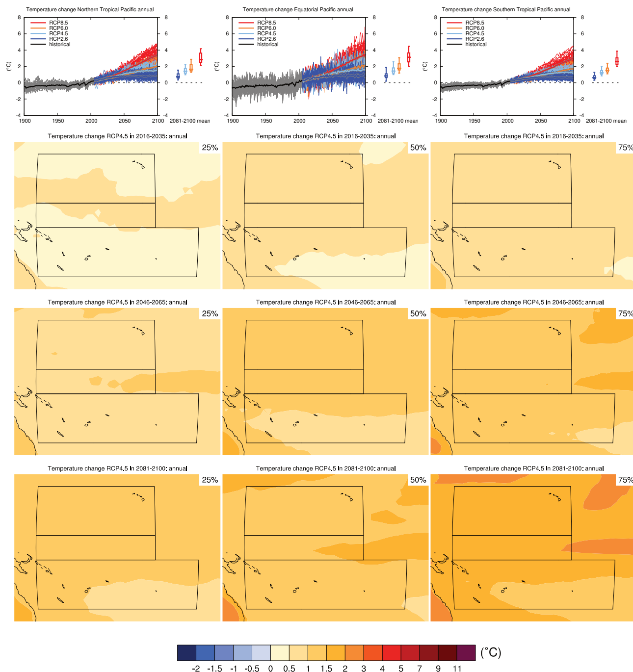
Figure AI.SM4.5.140 | (Top left) Time series of annual temperature change relative to 1986–2005 averaged over all grid points in the Northern Tropical Pacific (5°N to 25°N, 155°E to 150°W). Top middle | same for all grid points in the Equatorial Pacific (5°S to 5°N, 155°E to 150°W). (Top right) Same for all grid points in the Southern Tropical Pacific (5°S to 5°N, 155°E to 150°W). Thin lines denote one ensemble member per model, thick lines the CMIP5 multi-model mean. On the right-hand side the 5th, 25th, 50th (median), 75th and 95th percentiles of the distribution of 20-year mean changes are given for 2081–2100 in the four RCP scenarios.
