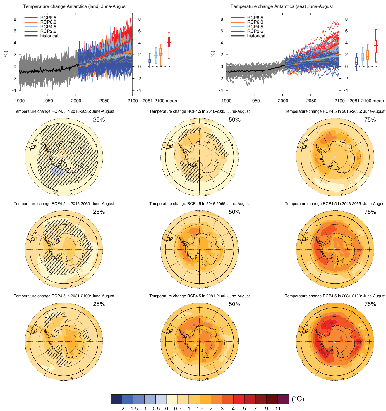
Figure AI.SM4.5.151 | (Top left) Time series of temperature change relative to 1986–2005 averaged over land grid points in Antarctica (90°S to 50°S) in June to August. (Top right) Same for sea grid points. Thin lines denote one ensemble member per model, thick lines the CMIP5 multi-model mean. On the right-hand side the 5th, 25th, 50th (median), 75th and 95th percentiles of the distribution of 20-year mean changes are given for 2081–2100 in the four RCP scenarios.
