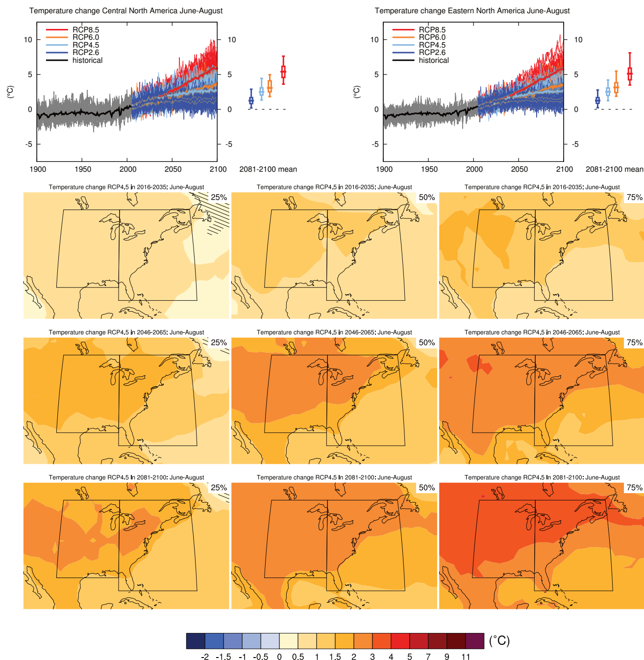
Figure AI.SM4.5.39 | (Top left) Time series of temperature change relative to 1986–2005 averaged over land grid points in Central North America (28.6°N to 50°N, 105°W to 85°W) in June to August. (Top right) Same for land grid points in Eastern North America (25°N to 50°N, 85°W to 60°W). Thin lines denote one ensemble member per model, thick lines the CMIP5 multi-model mean. On the right-hand side the 5th, 25th, 50th (median), 75th and 95th percentiles of the distribution of 20-year mean changes are given for 2081–2100 in the four RCP scenarios.
