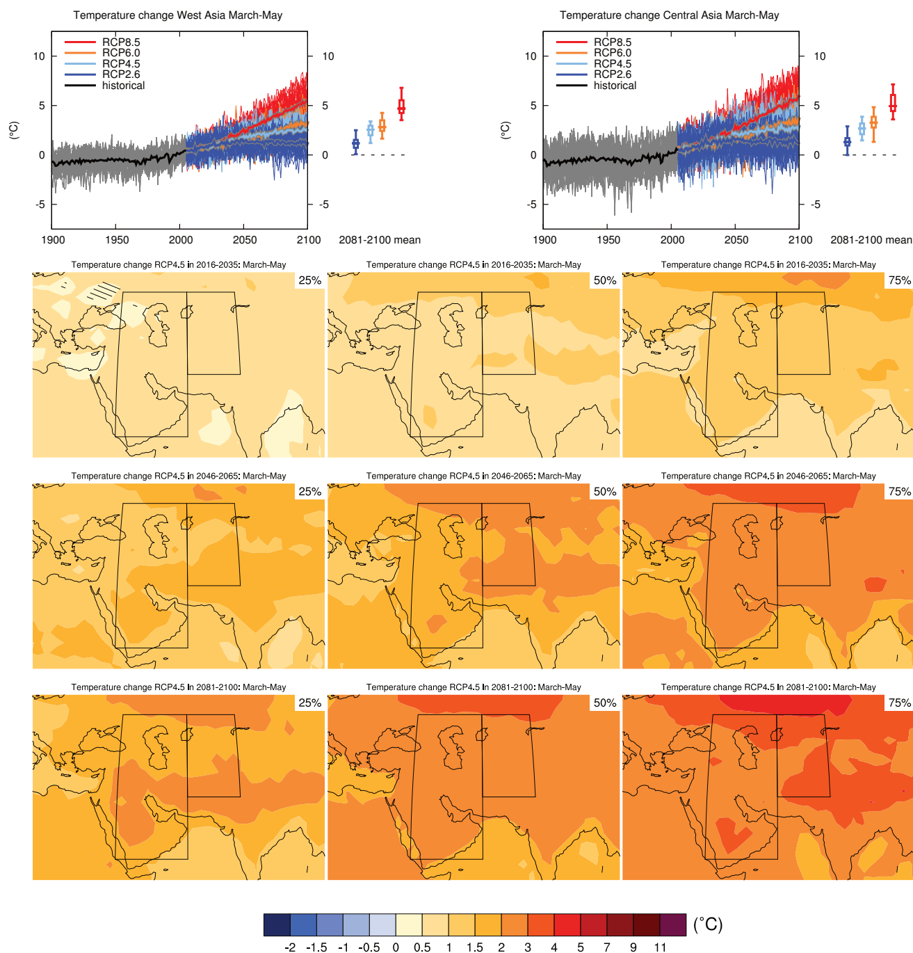
Figure AI.SM4.5.102 | (Top left) Time series of temperature change relative to 1986–2005 averaged over land grid points in West Asia (15°N to 50°N, 40°E to 60°E) in March to May. (Top right) Same for land grid points in Central Asia (30°N to 50°N, 60°E to 75°E). Thin lines denote one ensemble member per model, thick lines the CMIP5 multi-model mean. On the right-hand side the 5th, 25th, 50th (median), 75th and 95th percentiles of the distribution of 20-year mean changes are given for 2081–2100 in the four RCP scenarios.
