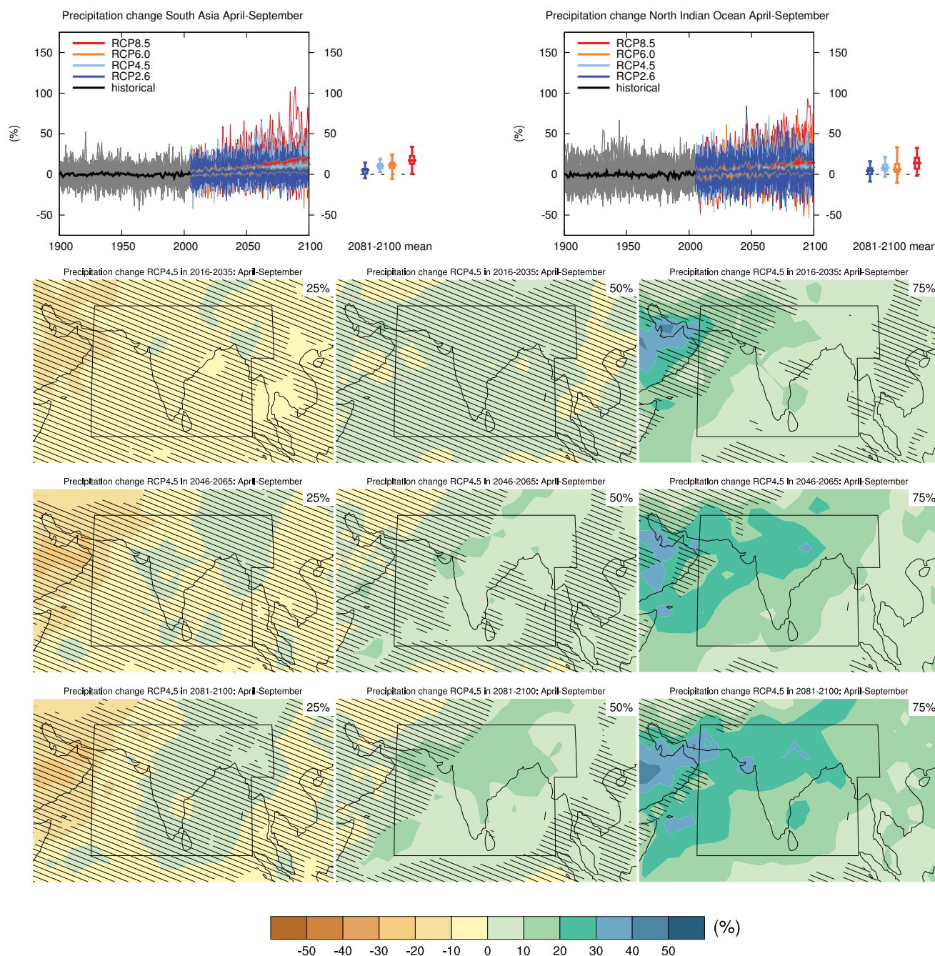
Figure AI.SM4.5.123 | (Top left) Time series of relative change relative to 1986–2005 in precipitation averaged over land grid points in South Asia (60°E, 5°N; 60°E, 30°N; 100°E, 30°N; 100°E, 20°E; 95°E, 20°N; 95°E, 5°N) in April to September. (Top right) Same for sea grid points in the North Indian Ocean (5°N to 30°N, 60°E to 95°E). Thin lines denote one ensemble member per model, thick lines the CMIP5 multi-model mean. On the right-hand side the 5th, 25th, 50th (median), 75th and 95th percentiles of the distribution of 20-year mean changes are given for 2081–2100 in the four RCP scenarios.
