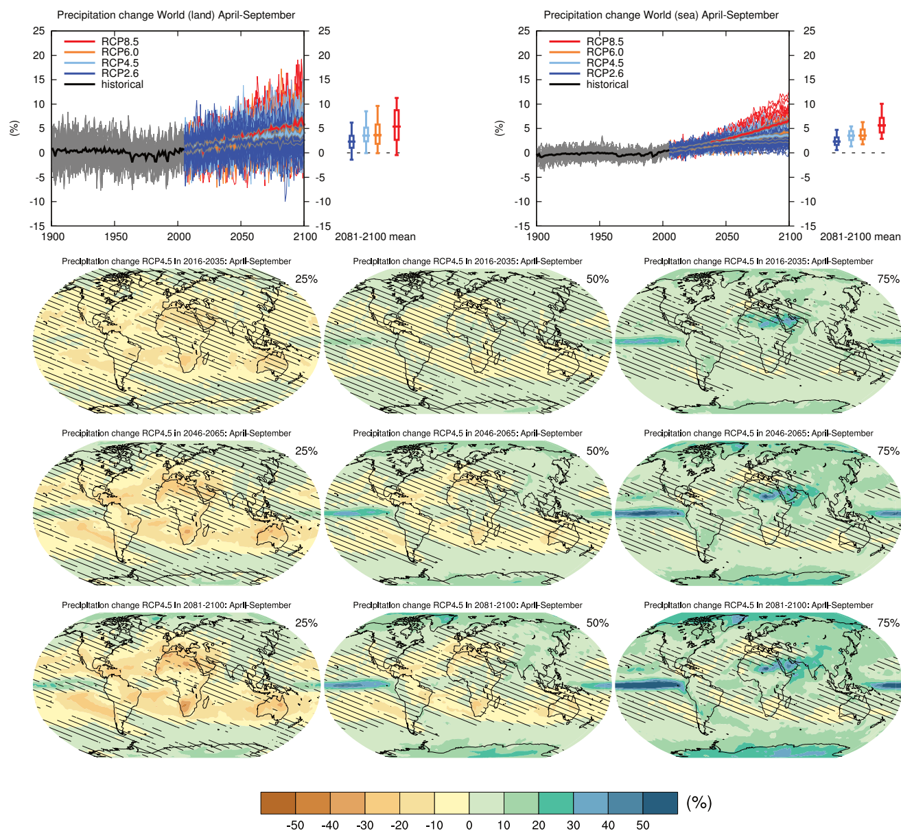
Figure AI.SM4.5.11 | (Top left) Time series of relative change relative to 1986–2005 in precipitation averaged over land grid points over the globe in April to September. (Top right) Same for sea grid points. Thin lines denote one ensemble member per model, thick lines the CMIP5 multi-model mean. On the right-hand side the 5th, 25th, 50th (median), 75th and 95th percentiles of the distribution of 20-year mean changes are given for 2081–2100 in the four RCP scenarios.
