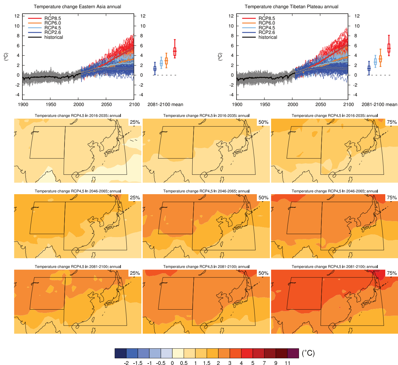
Figure AI.SM4.5.108 | (Top left) Time series of annual temperature change relative to 1986–2005 averaged over land grid points in Eastern Asia (20°N to 50°N, 100°E to 145°E). (Top right) Same for land grid points on the Tibetan Plateau (30°N to 50°N, 75°E to 100°E). Thin lines denote one ensemble member per model, thick lines the CMIP5 multi-model mean. On the right-hand side the 5th, 25th, 50th (median), 75th and 95th percentiles of the distribution of 20-year mean changes are given for 2081–2100 in the four RCP scenarios.
