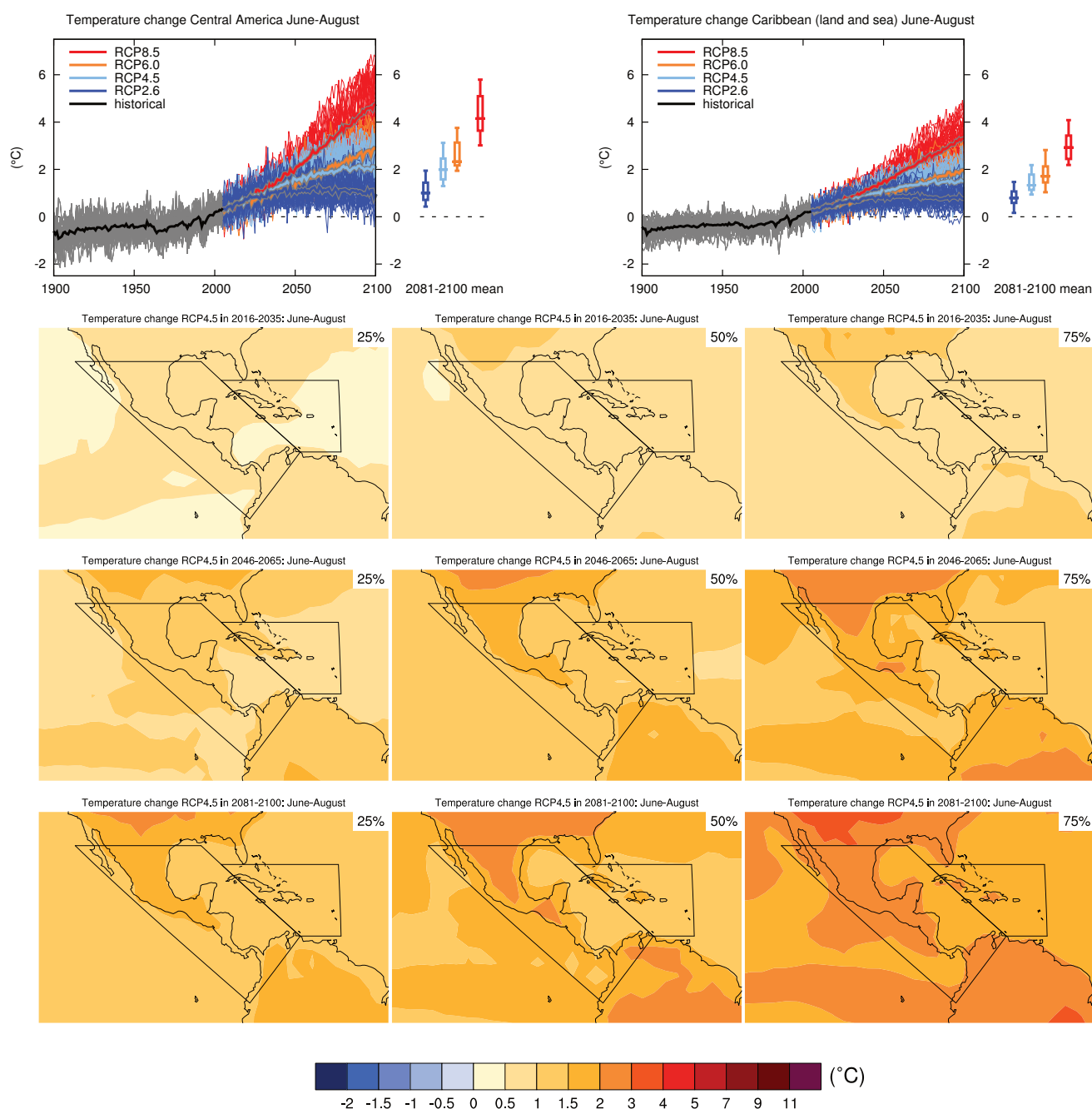
Figure AI.SM4.5.47 | (Top left) Time series of temperature change relative to 1986–2005 averaged over land grid points in Central America (68.8°W, 11.4°N; 79.7°W, 1.2°S; 116.3°W, 28.6°N; 90.3°W, 28.6°N) in June to August. (Top right) Same for all grid points in Caribbean (land and sea) (68.8°W, 11.4°N; 85.8°W, 25°N, 60°W, 25°N, 60°W, 11.44°N). Thin lines denote one ensemble member per model, thick lines the CMIP5 multi-model mean. On the right-hand side the 5th, 25th, 50th (median), 75th and 95th percentiles of the distribution of 20-year mean changes are given for 2081–2100 in the four RCP scenarios.
