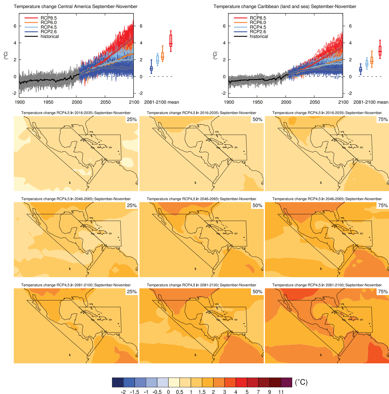
Figure AI.SM4.5.48 | (Top left) Time series of temperature change relative to 1986–2005 averaged over land grid points in Central America (68.8°W, 11.4°N; 79.7°W, 1.2°S; 116.3°W, 28.6°N; 90.3°W, 28.6°N) in September to November. (Top right) Same for all grid points in Caribbean (land and sea) (68.8°W, 11.4°N; 85.8°W, 25°N, 60°W, 25°N, 60°W, 11.44°N). Thin lines denote one ensemble member per model, thick lines the CMIP5 multi-model mean. On the right-hand side the 5th, 25th, 50th (median), 75th and 95th percentiles of the distribution of 20-year mean changes are given for 2081–2100 in the four RCP scenarios.
