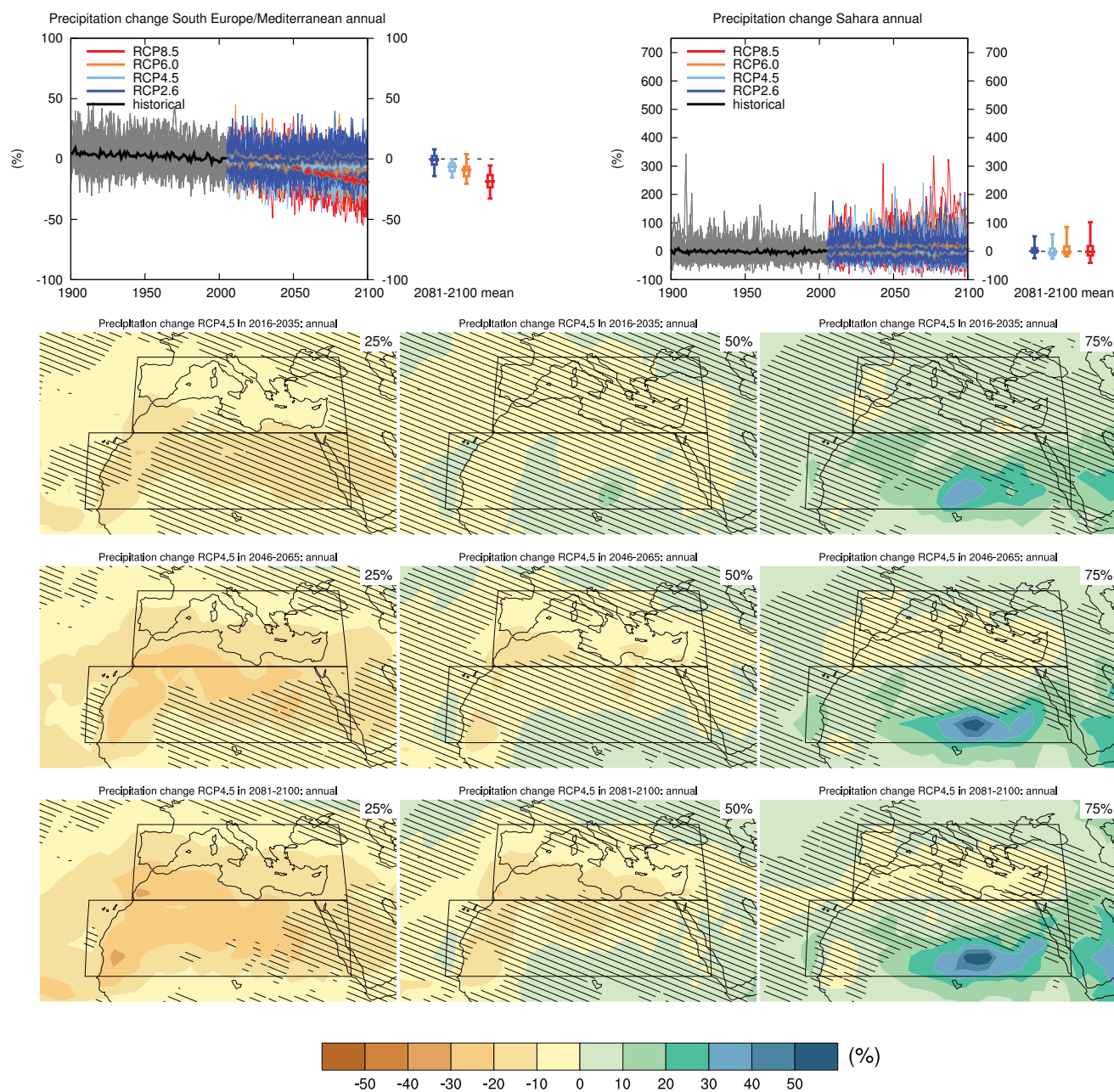
Figure AI.SM4.5.81 | (Top left) Time series of relative change relative to 1986–2005 in annual precipitation averaged over land grid points in the region South Europe/Mediterranean (30°N to 45°N, 10°W to 40°E). (Top right) Same for land grid points in the Sahara (15°N to 30°N, 20°W to 40°E). Thin lines denote one ensemble member per model, thick lines the CMIP5 multi-model mean. On the right-hand side the 5th, 25th, 50th (median), 75th and 95th percentiles of the distribution of 20-year mean changes are given for 2081–2100 in the four RCP scenarios. Note different scales.
