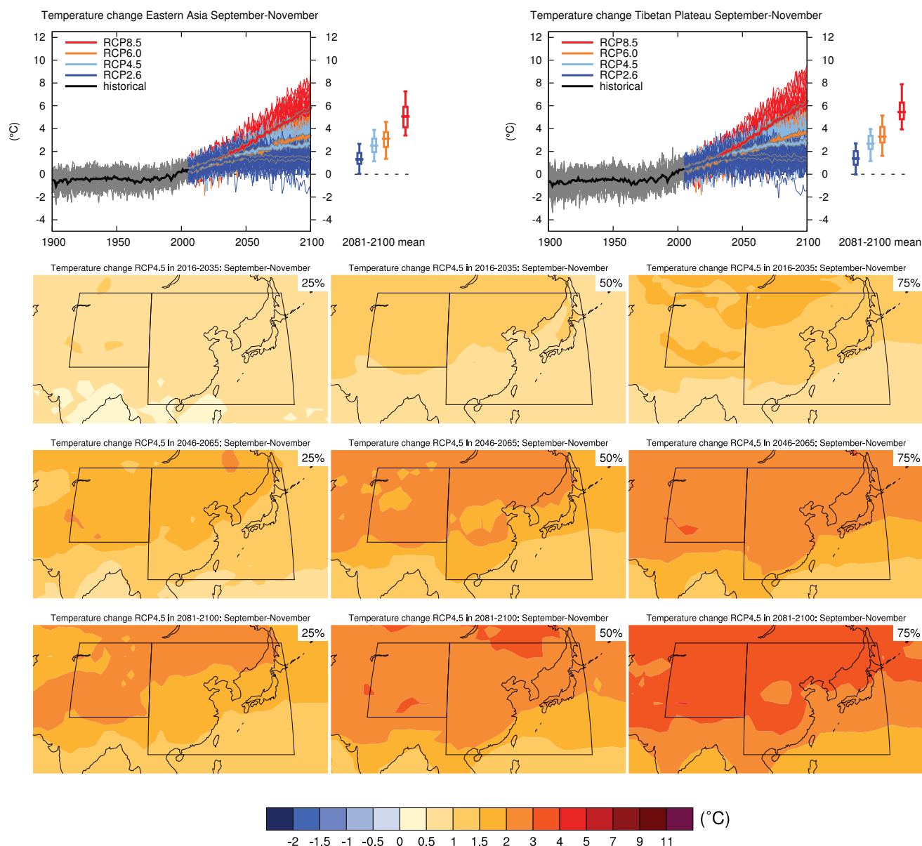
Figure AI.SM4.5.112 | (Top left) Time series of temperature change relative to 1986–2005 averaged over land grid points in Eastern Asia (20°N to 50°N, 100°E to 145°E) in September to November. (Top right) Same for land grid points on the Tibetan Plateau (30°N to 50°N, 75°E to 100°E). Thin lines denote one ensemble member per model, thick lines the CMIP5 multi-model mean. On the right-hand side the 5th, 25th, 50th (median), 75th and 95th percentiles of the distribution of 20-year mean changes are given for 2081–2100 in the four RCP scenarios.
