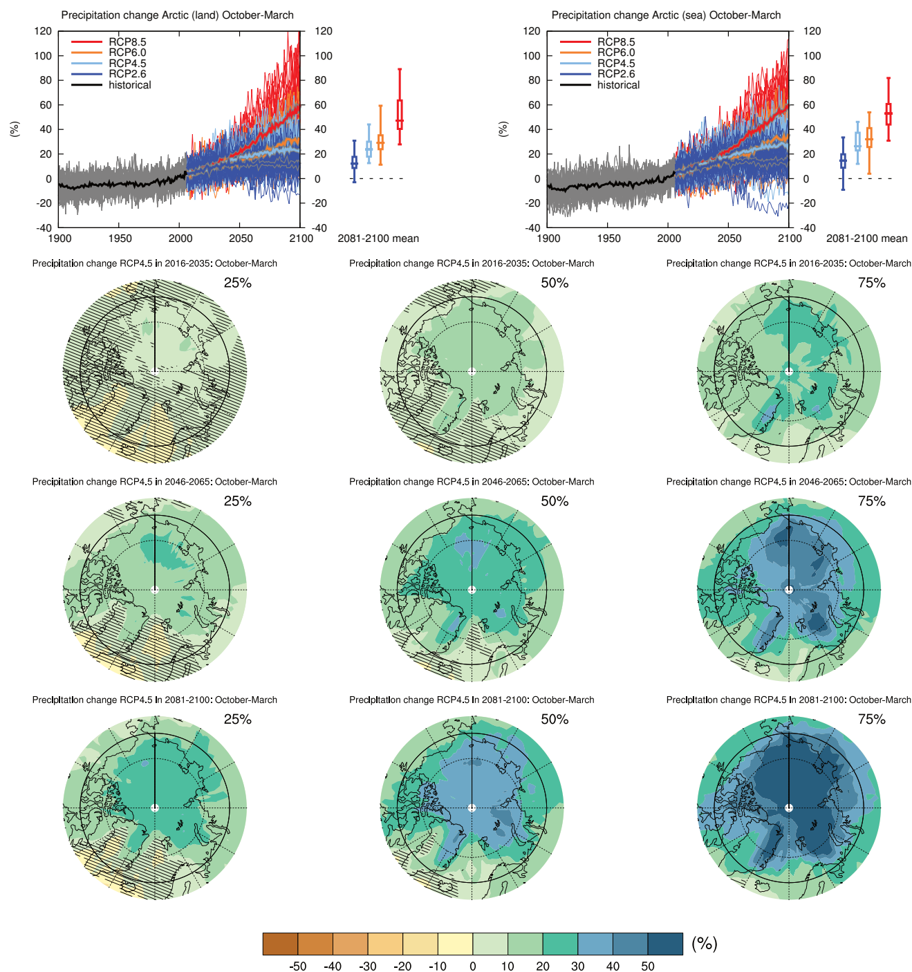
Figure AI.SM4.5.18 | (Top left) Time series of relative change relative to 1986–2005 in precipitation averaged over land grid points in the Arctic (67.5°N to 90°N) in October to March. (Top right) Same for sea grid points. Thin lines denote one ensemble member per model, thick lines the CMIP5 multi-model mean. On the right-hand side the 5th, 25th, 50th (median), 75th and 95th percentiles of the distribution of 20-year mean changes are given for 2081–2100 in the four RCP scenarios.
