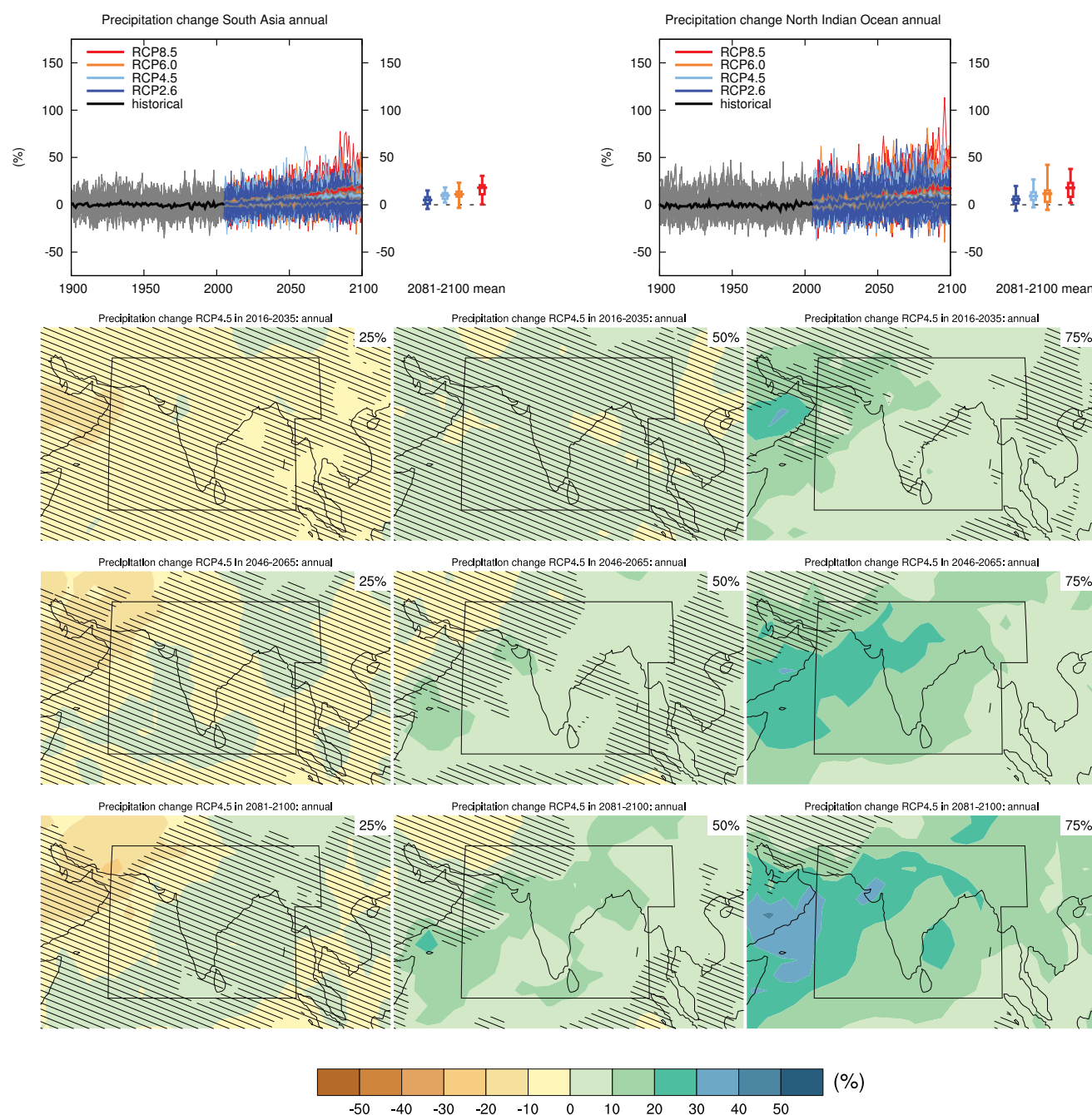
Figure AI.SM4.5.121 | (Top left) Time series of relative change relative to 1986–2005 in annual precipitation averaged over land grid points in South Asia (60°E, 5°N; 60°E, 30°N; 100°E, 30°N; 100°E, 20°E; 95°E, 20°N; 95°E, 5°N). (Top right) Same for sea grid points in the North Indian Ocean (5°N to 30°N, 60°E to 95°E). Thin lines denote one ensemble member per model, thick lines the CMIP5 multi-model mean. On the right-hand side the 5th, 25th, 50th (median), 75th and 95th percentiles of the distribution of 20-year mean changes are given for 2081–2100 in the four RCP scenarios.
