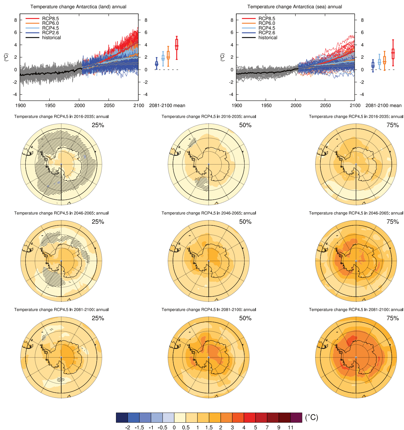
Figure AI.SM4.5.148 | (Top left) Time series of annual temperature change relative to 1986–2005 averaged over land grid points in Antarctica (90°S to 50°S). (Top right) Same for sea grid points. Thin lines denote one ensemble member per model, thick lines the CMIP5 multi-model mean. On the right-hand side the 5th, 25th, 50th (median), 75th and 95th percentiles of the distribution of 20-year mean changes are given for 2081–2100 in the four RCP scenarios.
