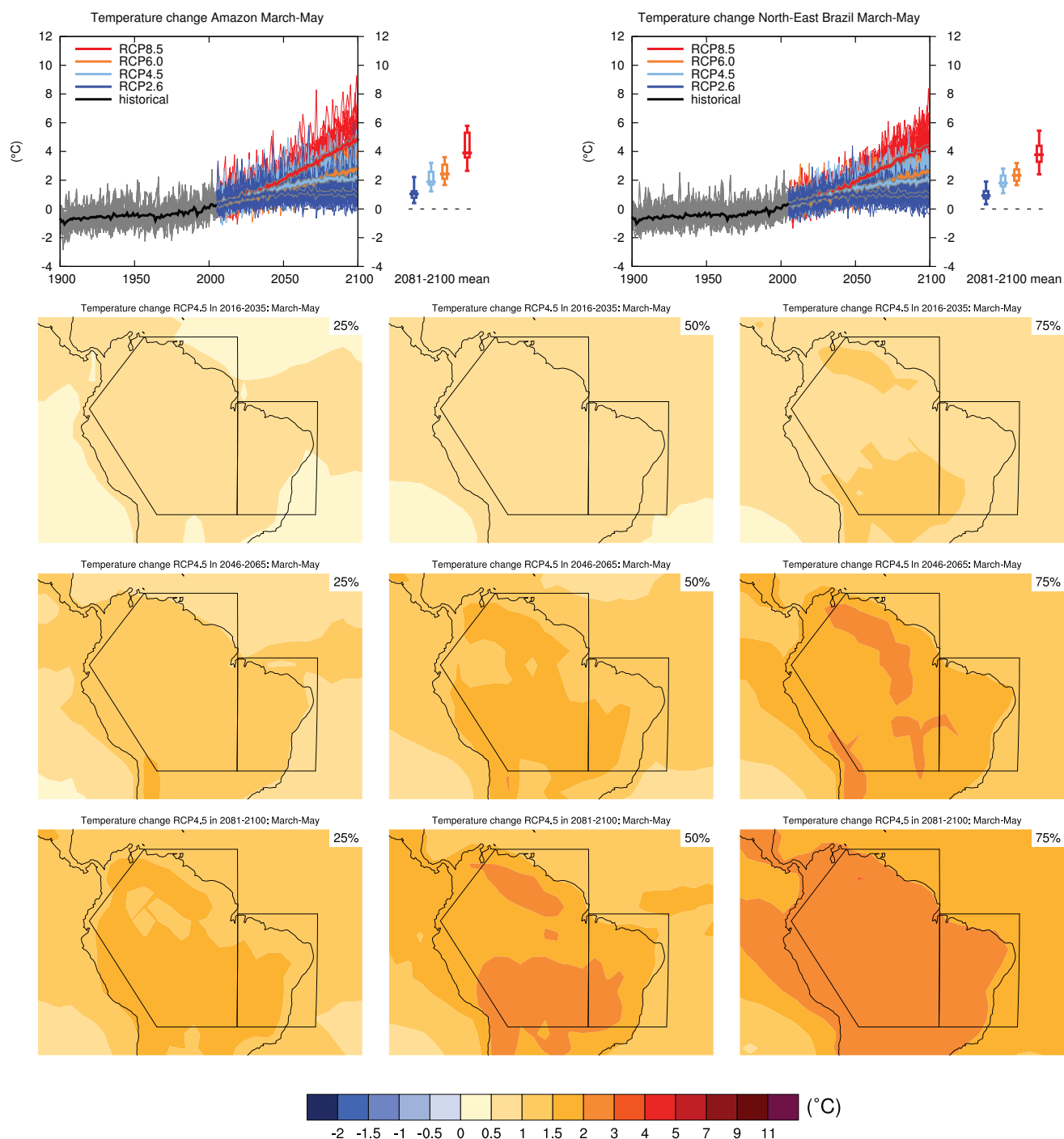
Figure AI.SM4.5.54 | (Top left) Time series of temperature change relative to 1986–2005 averaged over land grid points in the Amazon (20°S, 66.4°W; 1.24°S, 79.7°W; 11.44°N, 68.8°W; 11.44°N, 50°W; 20°S, 50°W) in March to May. (Top right) Same for land grid points in northeast Brazil (20°S to EQ, 50°W to 34°W). Thin lines denote one ensemble member per model, thick lines the CMIP5 multi-model mean. On the right-hand side the 5th, 25th, 50th (median), 75th and 95th percentiles of the distribution of 20-year mean changes are given for 2081–2100 in the four RCP scenarios.
