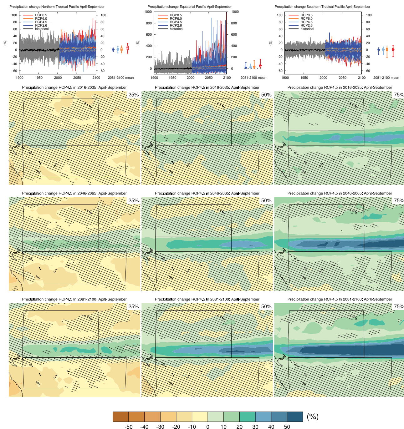
Figure AI.SM4.5.147 | (Top left) Time series of relative change relative to 1986–2005 in precipitation averaged over all grid points in the Northern Tropical Pacific (5°N to 25°N, 155°E to 150°W) in April to September. Top middle | same for all grid points in the Equatorial Pacific (5°S to 5°N, 155°E to 150°W). (Top right) Same for all grid points in the Southern Tropical Pacific (5°S to 5°N, 155°E to 150°W). Thin lines denote one ensemble member per model, thick lines the CMIP5 multi-model mean. On the right-hand side the 5th, 25th, 50th (median), 75th and 95th percentiles of the distribution of 20-year mean changes are given for 2081–2100 in the four RCP scenarios. Note different scales.
