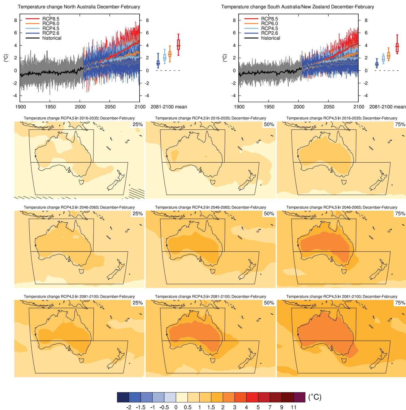
Figure AI.SM4.5.133 | (Top left) Time series of temperature change relative to 1986–2005 averaged over land grid points in North Australia (30°S to 10°S, 110°E to 155°E) in December to February. (Top right) Same for land grid points in South Australia/New Zealand (50°S to 30°S, 110°E to 180°E). Thin lines denote one ensemble member per model, thick lines the CMIP5 multi-model mean. On the right-hand side the 5th, 25th, 50th (median), 75th and 95th percentiles of the distribution of 20-year mean changes are given for 2081–2100 in the four RCP scenarios.
