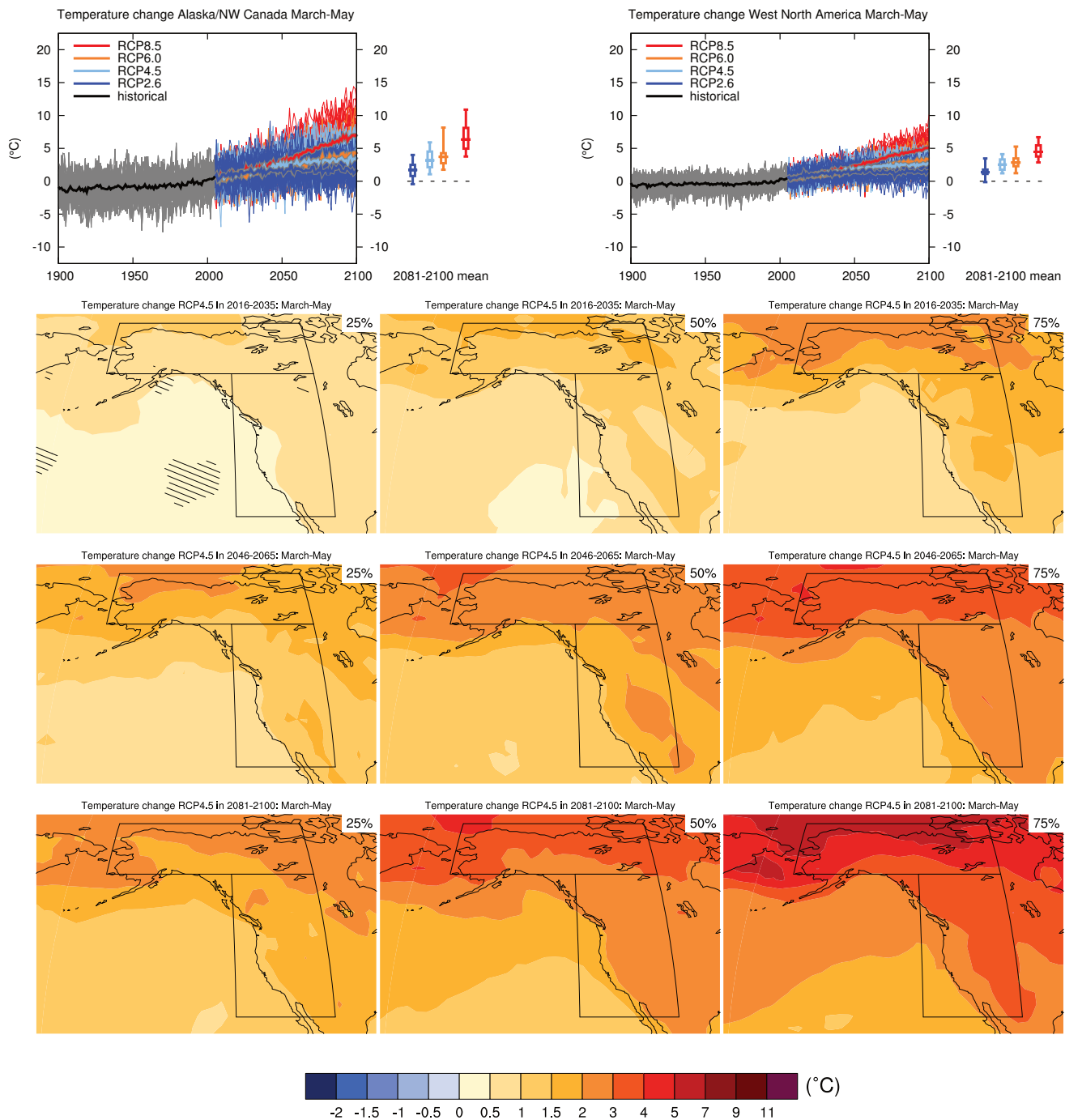
Figure AI.SM4.5.30 | (Top left) Time series of temperature change relative to 1986–2005 averaged over land grid points in Alaska/NW Canada (60°N to 72.6°N, 168°W to 105°W) in March to May. (Top right) Same for land grid points in West North America (28.6°N to 60°N, 130°W to 105°W). Thin lines denote one ensemble member per model, thick lines the CMIP5 multi-model mean. On the right-hand side the 5th, 25th, 50th (median), 75th and 95th percentiles of the distribution of 20-year mean changes are given for 2081–2100 in the four RCP scenarios.
