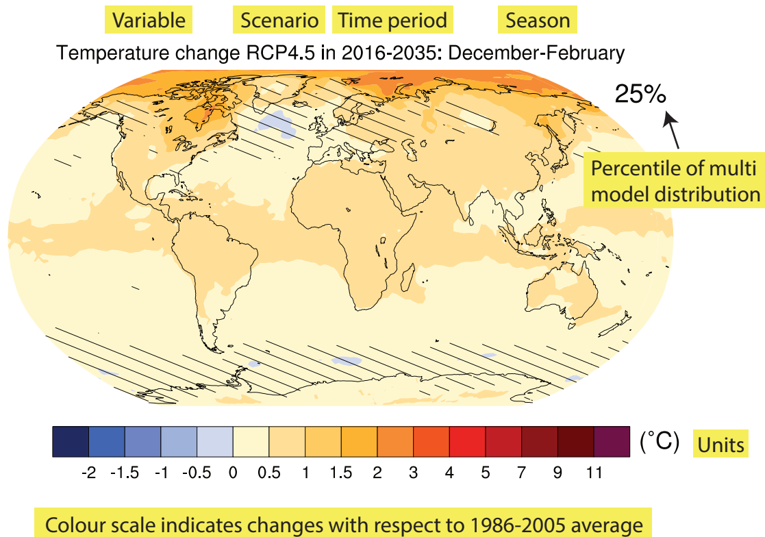
Figure AI.SM4.5.2 | Explanation of the features of a typical spatial map presented in Annex I. Hatching indicates regions where the magnitude of the 25th, median or 75th percentile of the 20-year mean change is less than 1 standard deviation of model-estimated natural variability of 20-year mean differences.
