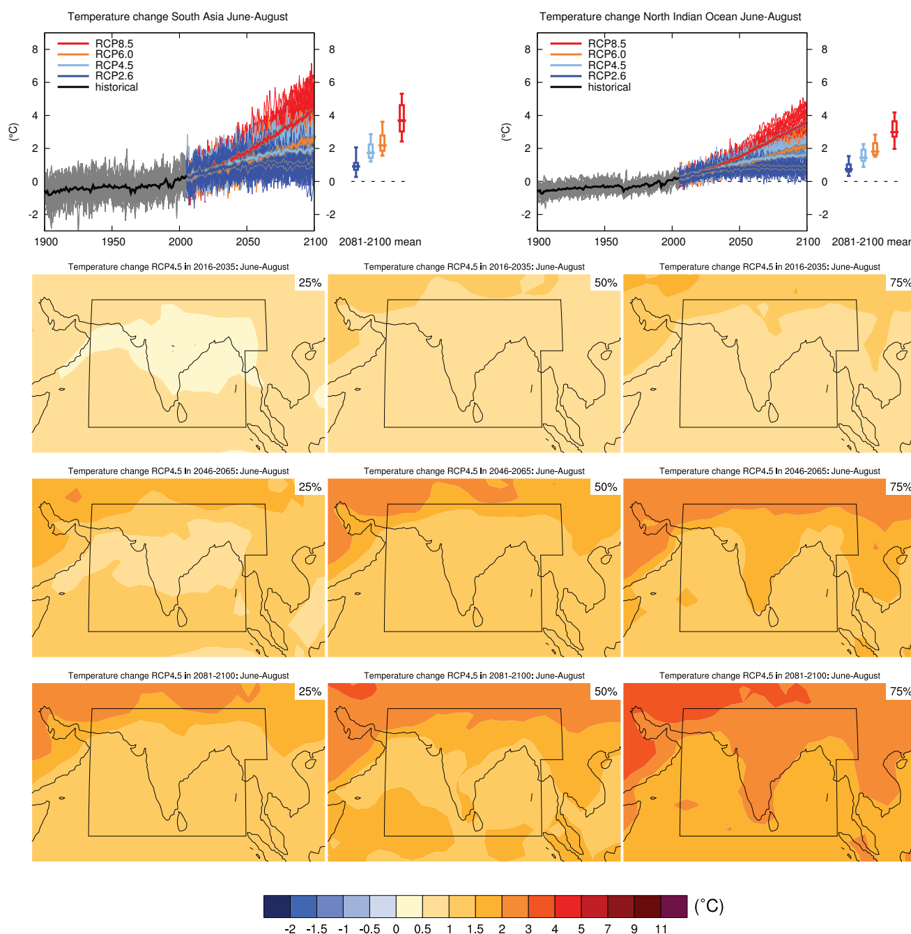
Figure AI.SM4.5.119 | (Top left) Time series of temperature change relative to 1986–2005 averaged over land grid points in South Asia (60°E, 5°N; 60°E, 30°N; 100°E, 30°N; 100°E, 20°E; 95°E, 20°N; 95°E, 5°N) in June to August. (Top right) Same for sea grid points in the North Indian Ocean (5°N to 30°N, 60°E to 95°E). Thin lines denote one ensemble member per model, thick lines the CMIP5 multi-model mean. On the right-hand side the 5th, 25th, 50th (median), 75th and 95th percentiles of the distribution of 20-year mean changes are given for 2081–2100 in the four RCP scenarios.
