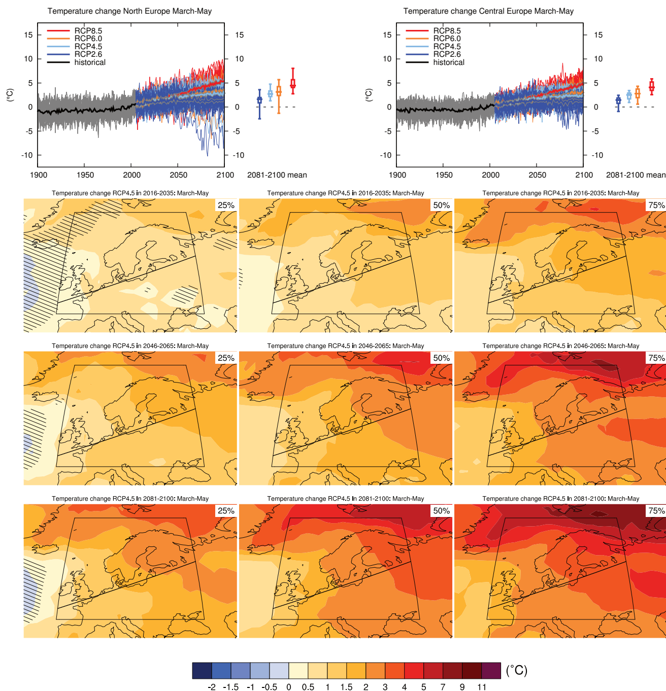
Figure AI.SM4.5.70 | (Top left) Time series of temperature change relative to 1986–2005 averaged over land grid points in North Europe (10°W,48°N; 10°W,75°N; 40°E,75°N; 40°E,61.3°N) in March to May. (Top right) Same for land grid points in Central Europe (10°W, 45°N; 10°W,48°N; 40°E, 61.3°N; 40°E,45°N). Thin lines denote one ensemble member per model, thick lines the CMIP5 multi-model mean. On the right-hand side the 5th, 25th, 50th (median), 75th and 95th percentiles of the distribution of 20-year mean changes are given for 2081–2100 in the four RCP scenarios.
