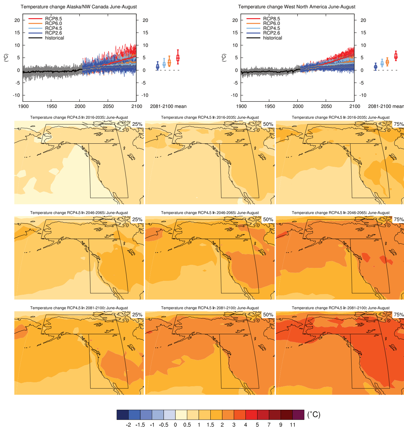
Figure AI.SM4.5.31 | (Top left) Time series of temperature change relative to 1986–2005 averaged over land grid points in Alaska/NW Canada (60°N to 72.6°N, 168°W to 105°W) in June to August. (Top right) Same for land grid points in West North America (28.6°N to 60°N, 130°W to 105°W). Thin lines denote one ensemble member per model, thick lines the CMIP5 multi-model mean. On the right-hand side the 5th, 25th, 50th (median), 75th and 95th percentiles of the distribution of 20-year mean changes are given for 2081–2100 in the four RCP scenarios.
