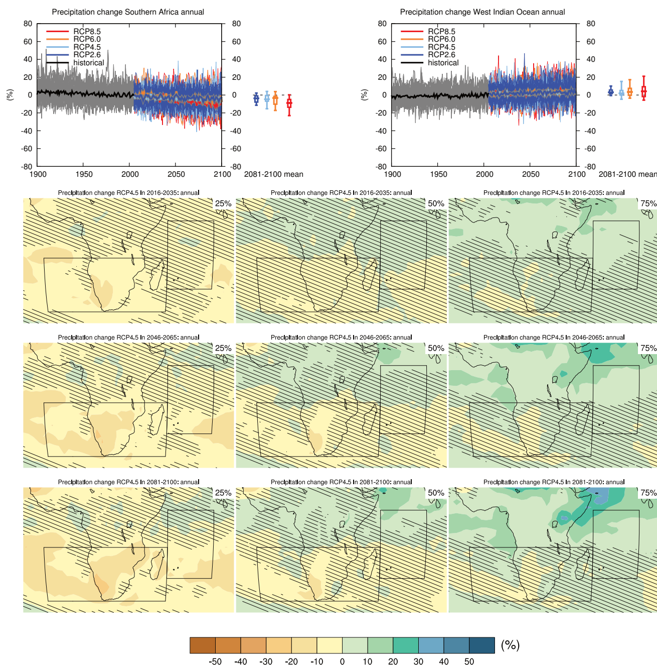
Figure AI.SM4.5.97 | (Top left) Time series of relative change relative to 1986–2005 in annual precipitation averaged over land grid points in Southern Africa (35°S to 11.4°S, 10°W to 52°E). (Top right) Same for sea grid points in the West Indian Ocean (25°S to 5°N, 52°E to 75°E). Thin lines denote one ensemble member per model, thick lines the CMIP5 multi-model mean. On the right-hand side the 5th, 25th, 50th (median), 75th and 95th percentiles of the distribution of 20-year mean changes are given for 2081–2100 in the four RCP scenarios.
