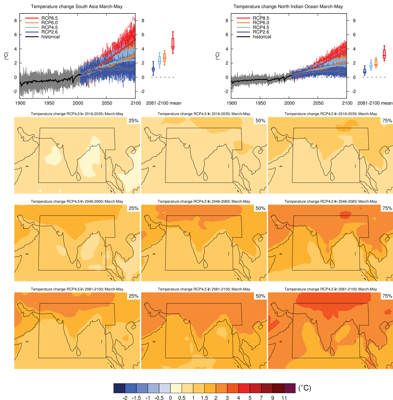
Figure AI.SM4.5.118 | (Top left) Time series of temperature change relative to 1986–2005 averaged over land grid points in South Asia (60°E, 5°N; 60°E, 30°N; 100°E, 30°N; 100°E, 20°E; 95°E, 20°N; 95°E, 5°N) in March to May. (Top right) Same for sea grid points in the North Indian Ocean (5°N to 30°N, 60°E to 95°E). Thin lines denote one ensemble member per model, thick lines the CMIP5 multi-model mean. On the right-hand side the 5th, 25th, 50th (median), 75th and 95th percentiles of the distribution of 20-year mean changes are given for 2081–2100 in the four RCP scenarios.
