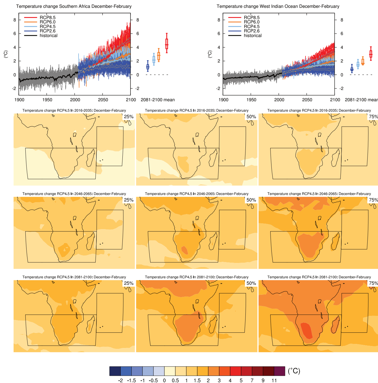
Figure AI.SM4.5.93 | (Top left) Time series of temperature change relative to 1986–2005 averaged over land grid points in Southern Africa (35°S to 11.4°S, 10°W to 52°E) in December to February. (Top right) Same for sea grid points in the West Indian Ocean (25°S to 5°N, 52°E to 75°E). Thin lines denote one ensemble member per model, thick lines the CMIP5 multi-model mean. On the right-hand side the 5th, 25th, 50th (median), 75th and 95th percentiles of the distribution of 20-year mean changes are given for 2081–2100 in the four RCP scenarios.
