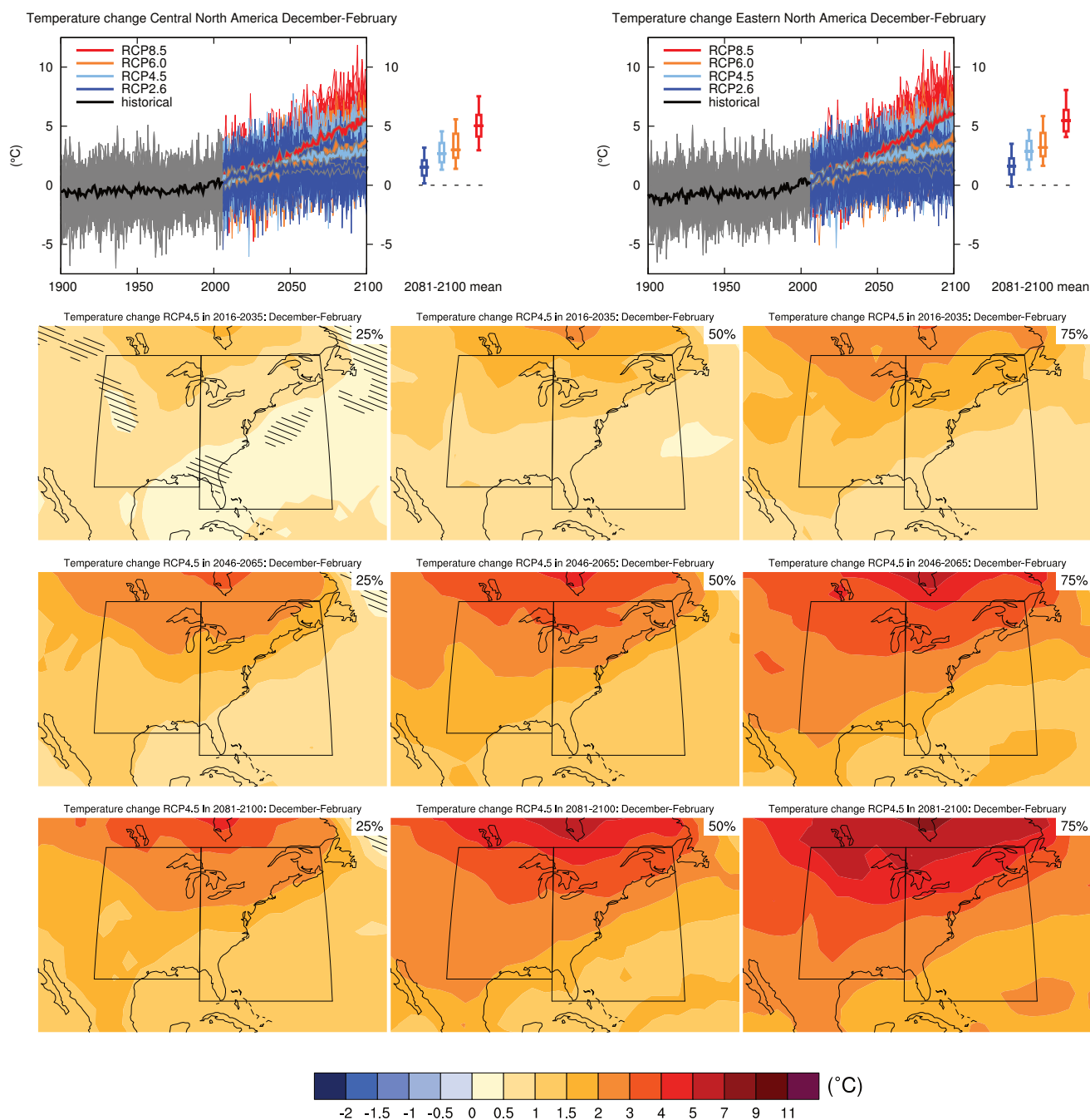
Figure AI.SM4.5.37 | (Top left) Time series of temperature change relative to 1986–2005 averaged over land grid points in Central North America (28.6°N to 50°N, 105°W to 85°W) in December to February. (Top right) Same for land grid points in Eastern North America (25°N to 50°N, 85°W to 60°W). Thin lines denote one ensemble member per model, thick lines the CMIP5 multi-model mean. On the right-hand side the 5th, 25th, 50th (median), 75th and 95th percentiles of the distribution of 20-year mean changes are given for 2081–2100 in the four RCP scenarios.
