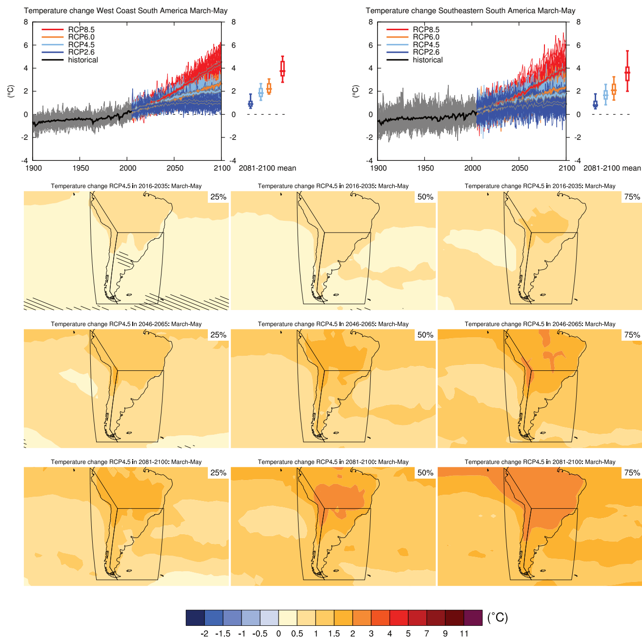
Figure AI.SM4.5.62 | (Top left) Time series of temperature change relative to 1986–2005 averaged over land grid points in the west coast of South America (79.7°W, 1.2°S; 66.4°W, 20°S; 72.1°W, 50°S; 67.3°W, 56.7°S; 82.0°W, 56.7°S; 82.2°W, 0.5°N) in March to May. (Top right) Same for land grid points in southeastern South America (39.4°W, 20°S; 39.4°W, 56.6°S; 67.3°W, 56.7°S; 72.1°W, 50°S; 66°W, 20°S). Thin lines denote one ensemble member per model, thick lines the CMIP5 multi-model mean. On the right-hand side the 5th, 25th, 50th (median), 75th and 95th percentiles of the distribution of 20-year mean changes are given for 2081–2100 in the four RCP scenarios.
