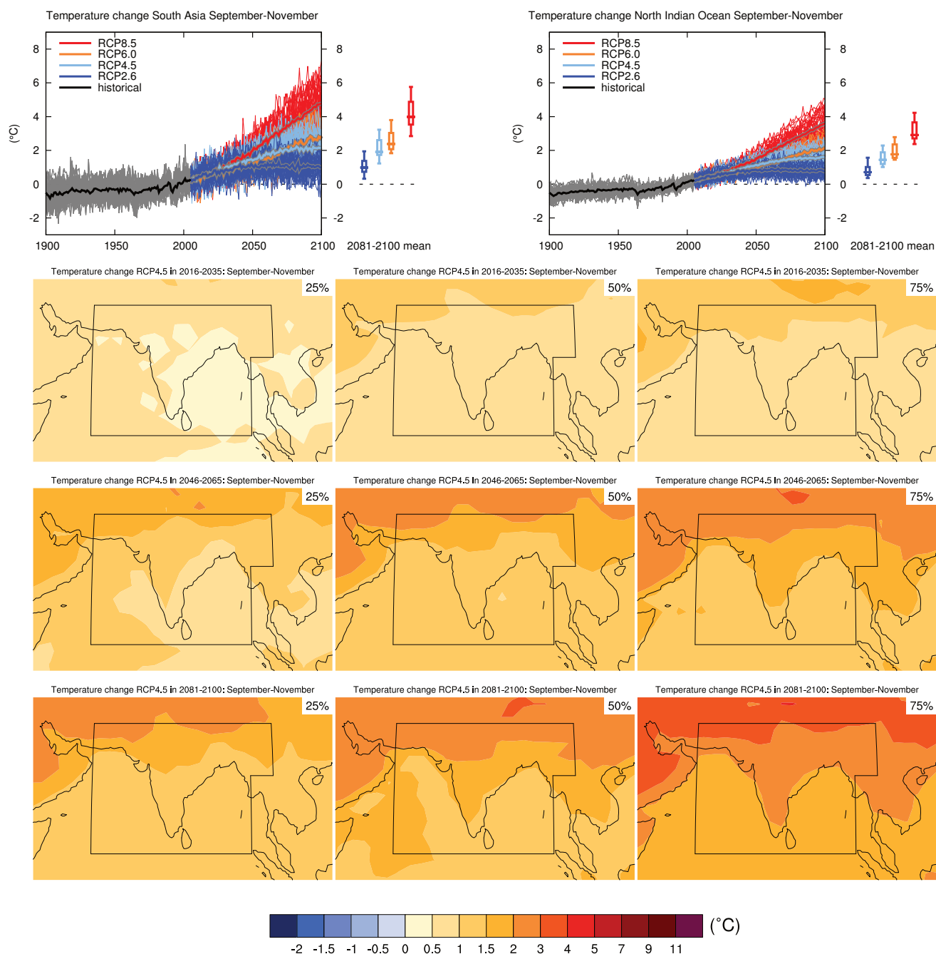
Figure AI.SM4.5.120 | (Top left) Time series of temperature change relative to 1986–2005 averaged over land grid points in South Asia (60°E, 5°N; 60°E, 30°N; 100°E, 30°N; 100°E, 20°E; 95°E, 20°N; 95°E, 5°N) in September to November. (Top right) Same for sea grid points in the North Indian Ocean (5°N to 30°N, 60°E to 95°E). Thin lines denote one ensemble member per model, thick lines the CMIP5 multi-model mean. On the right-hand side the 5th, 25th, 50th (median), 75th and 95th percentiles of the distribution of 20-year mean changes are given for 2081–2100 in the four RCP scenarios.
