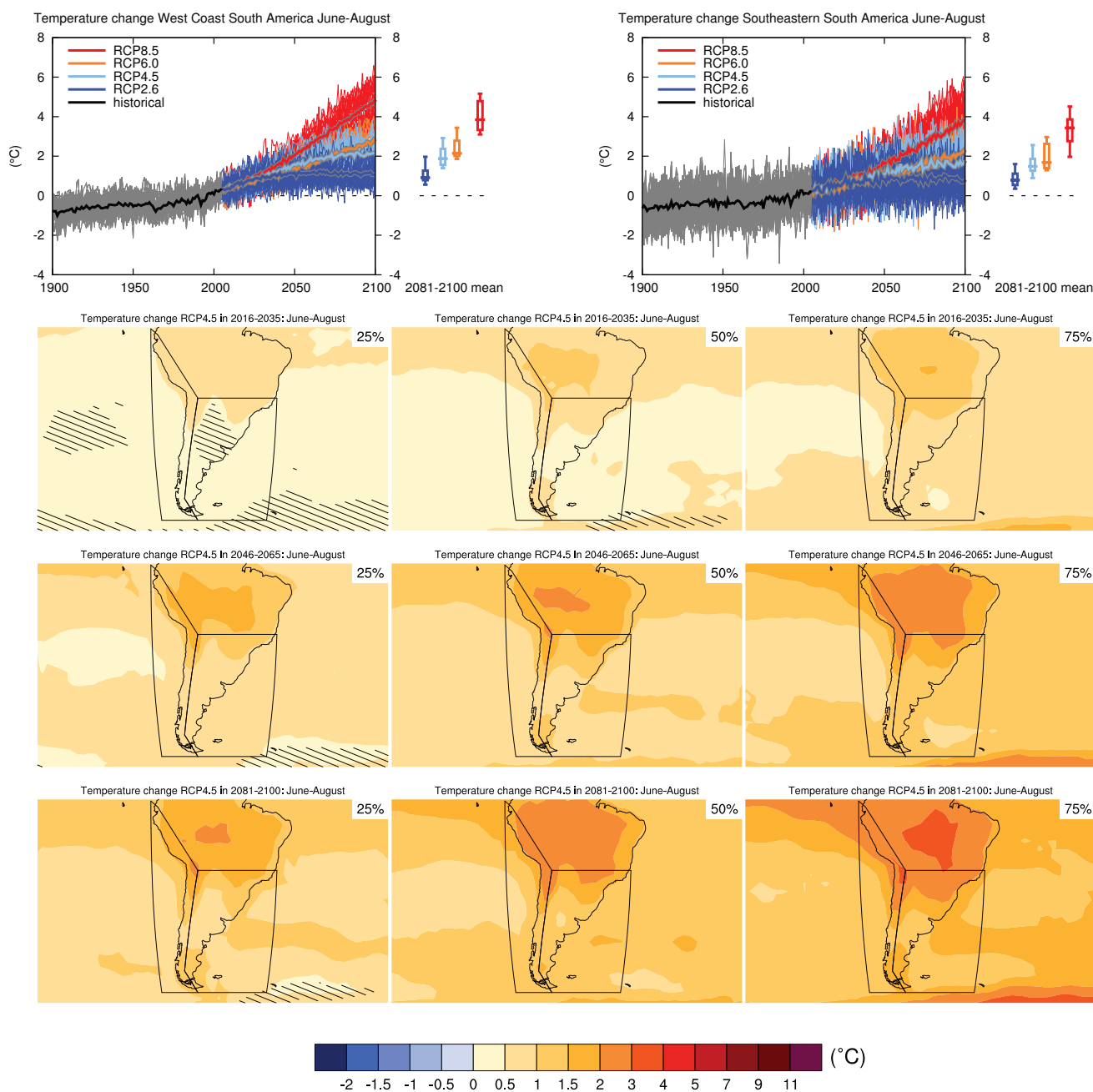
Figure AI.SM4.5.63 | (Top left) Time series of temperature change relative to 1986–2005 averaged over land grid points in the west coast of South America (79.7°W, 1.2°S; 66.4°W, 20°S; 72.1°W, 50°S; 67.3°W, 56.7°S; 82.0°W, 56.7°S; 82.2°W, 0.5°N) in June to August. (Top right) Same for land grid points in southeastern South America (39.4°W, 20°S; 39.4°W, 56.6°S; 67.3°W, 56.7°S; 72.1°W, 50°S; 66°W, 20°S). Thin lines denote one ensemble member per model, thick lines the CMIP5 multi-model mean. On the right-hand side the 5th, 25th, 50th (median), 75th and 95th percentiles of the distribution of 20-year mean changes are given for 2081–2100 in the four RCP scenarios.
