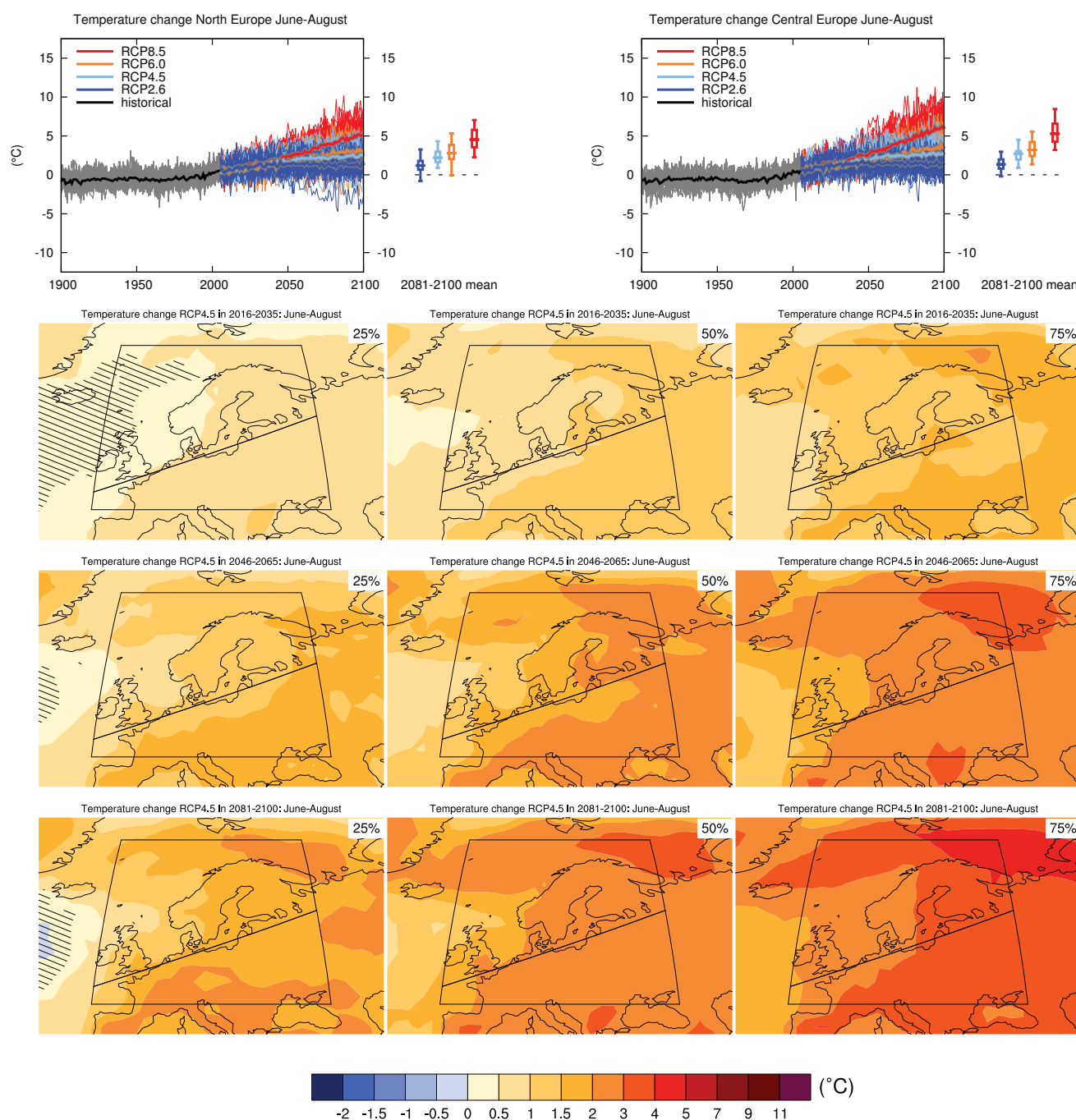
Figure AI.SM4.5.71 | (Top left) Time series of temperature change relative to 1986–2005 averaged over land grid points in North Europe (10°W, 48°N; 10°W, 75°N; 40°E, 75°N; 40°E, 61.3°N) in June to August. (Top right) Same for land grid points in Central Europe (10°W, 45°N; 10°W, 48°N; 40°E, 61.3°N; 40°E, 45°N). Thin lines denote one ensemble member per model, thick lines the CMIP5 multi-model mean. On the right-hand side the 5th, 25th, 50th (median), 75th and 95th percentiles of the distribution of 20-year mean changes are given for 2081–2100 in the four RCP scenarios.
