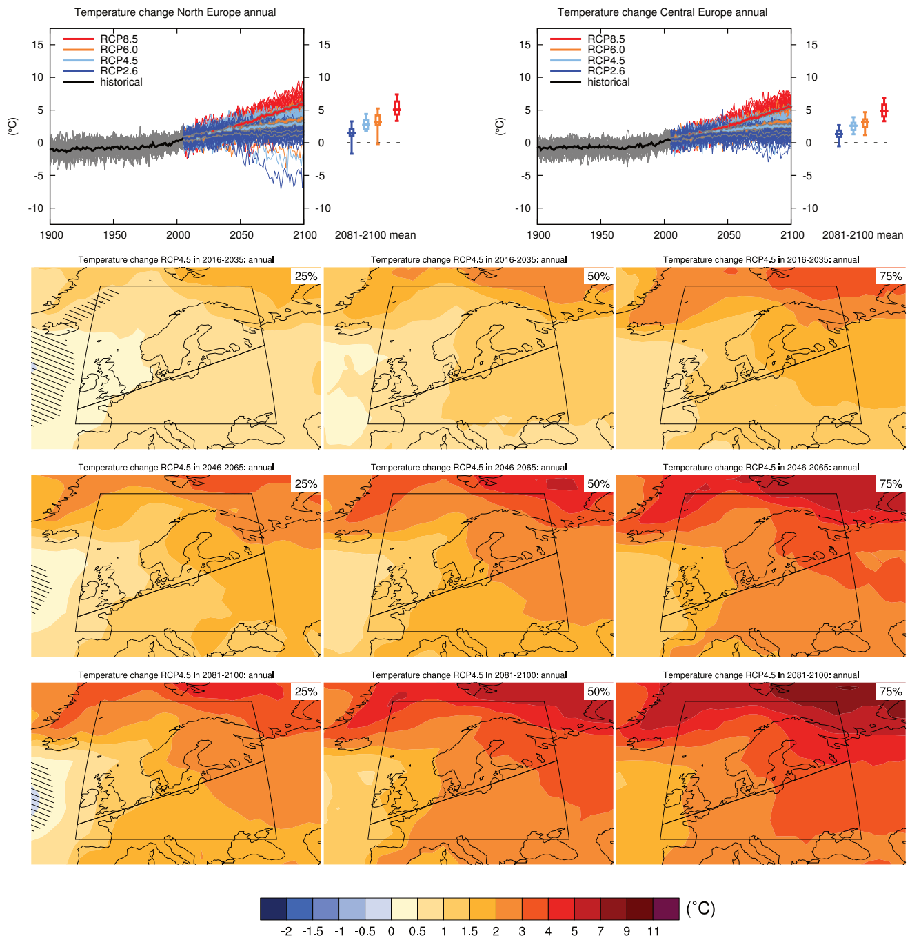
Figure AI.SM4.5.68 | (Top left) Time series of annual temperature change relative to 1986–2005 averaged over land grid points in North Europe (10°W, 48°N; 10°W, 75°N; 40°E, 75°N; 40°E, 61.3°N). (Top right) Same for land grid points in Central Europe (10°W, 45°N; 10°W, 48°N; 40°E, 61.3°N; 40°E, 45°N). Thin lines denote one ensemble member per model, thick lines the CMIP5 multi-model mean. On the right-hand side the 5th, 25th, 50th (median), 75th and 95th percentiles of the distribution of 20-year mean changes are given for 2081–2100 in the four RCP scenarios.
