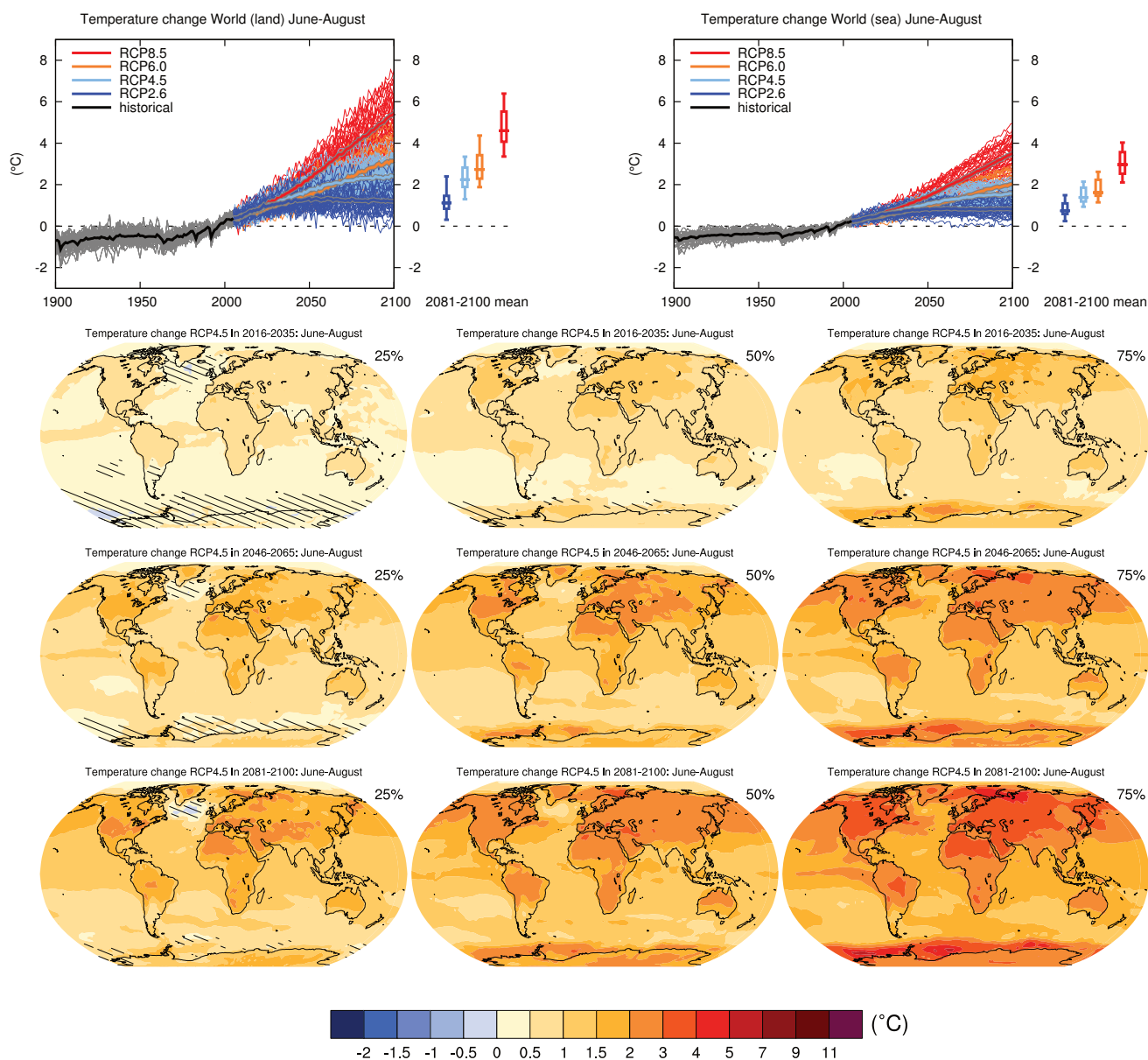
Figure AI.SM4.5.7 | (Top left) Time series of temperature change relative to 1986–2005 averaged over land grid points over the globe in June to August. (Top right) Same for sea grid points. Thin lines denote one ensemble member per model, thick lines the CMIP5 multi-model mean. On the right-hand side the 5th, 25th, 50th (median), 75th and 95th percentiles of the distribution of 20-year mean changes are given for 2081–2100 in the four RCP scenarios.
