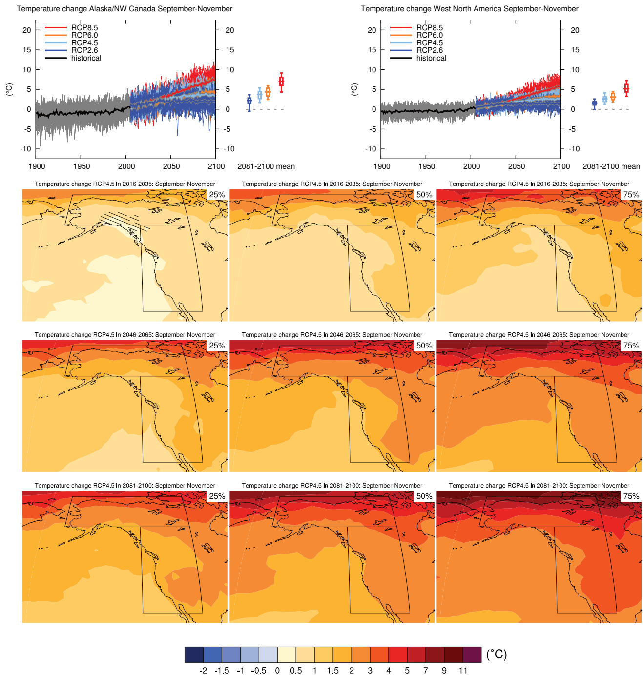
Figure AI.SM4.5.32 | (Top left) Time series of temperature change relative to 1986–2005 averaged over land grid points in Alaska/NW Canada (60°N to 72.6°N, 168°W to 105°W) in September to November. (Top right) Same for land grid points in West North America (28.6°N to 60°N, 130°W to 105°W). Thin lines denote one ensemble member per model, thick lines the CMIP5 multi-model mean. On the right-hand side the 5th, 25th, 50th (median), 75th and 95th percentiles of the distribution of 20-year mean changes are given for 2081–2100 in the four RCP scenarios.
