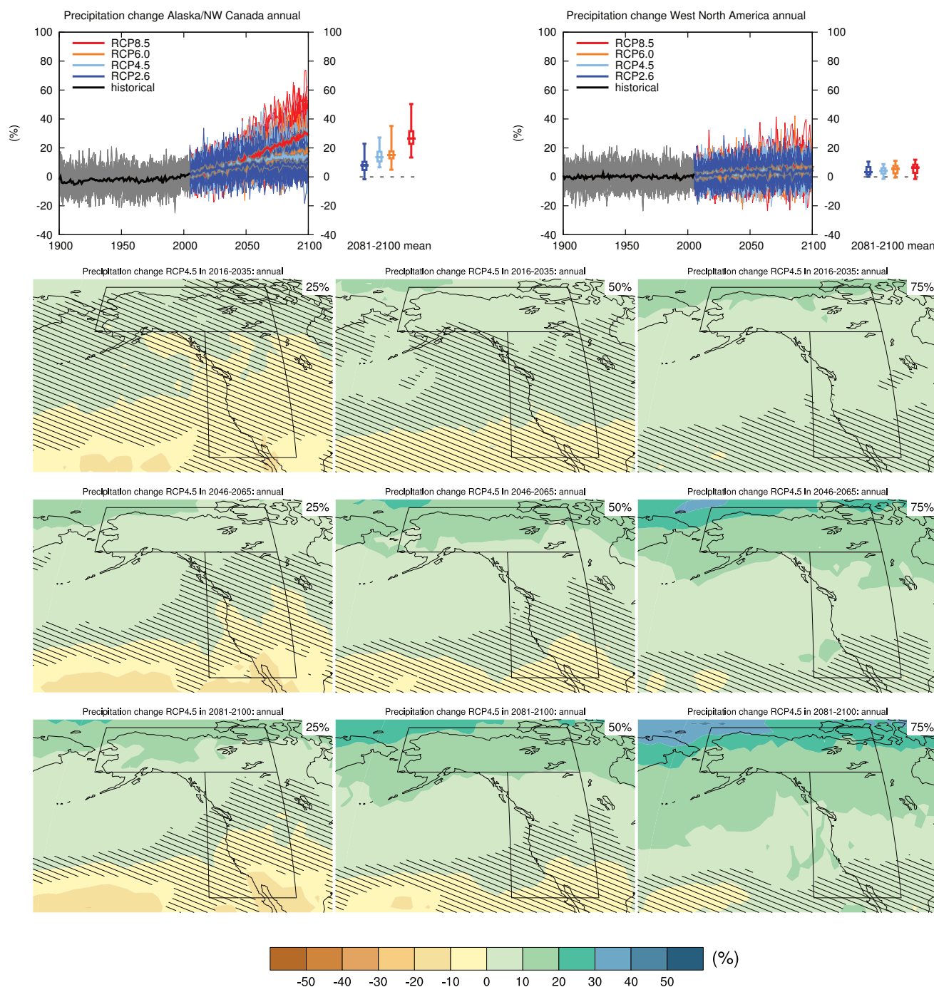
Figure AI.SM4.5.33 | (Top left) Time series of relative change relative to 1986–2005 in annual precipitation averaged over land grid points in Alaska/NW Canada (60°N to 72.6°N, 168°W to 105°W). (Top right) Same for land grid points in West North America (28.6°N to 60°N, 130°W to 105°W). Thin lines denote one ensemble member per model, thick lines the CMIP5 multi-model mean. On the right-hand side the 5th, 25th, 50th (median), 75th and 95th percentiles of the distribution of 20-year mean changes are given for 2081–2100 in the four RCP scenarios.
