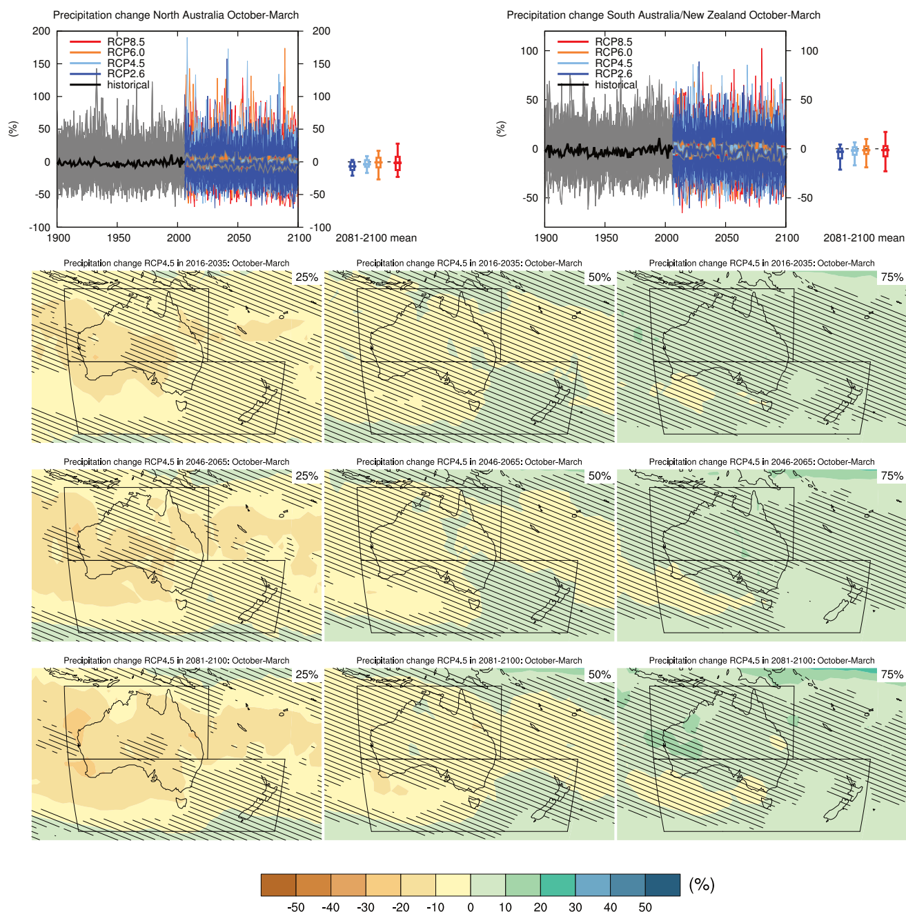
Figure AI.SM4.5.138 | (Top left) Time series of relative change relative to 1986–2005 in precipitation averaged over land grid points in North Australia (30°S to 10°S, 110°E to 155°E) in October to March. (Top right) Same for land grid points in South Australia/New Zealand (50°S to 30°S, 110°E to 180°E). Thin lines denote one ensemble member per model, thick lines the CMIP5 multi-model mean. On the right-hand side the 5th, 25th, 50th (median), 75th and 95th percentiles of the distribution of 20-year mean changes are given for 2081–2100 in the four RCP scenarios. Note different scales.
