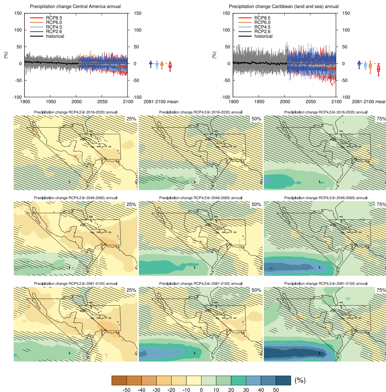
Figure AI.SM4.5.49 | (Top left) Time series of relative change relative to 1986–2005 in annual precipitation averaged over land grid points in Central America (68.8°W, 11.4°N; 79.7°W, 1.2°S; 116.3°W, 28.6°N; 90.3°W, 28.6°N). (Top right) Same for all grid points in Caribbean (land and sea) (68.8°W, 11.4°N; 85.8°W, 25°N, 60°W, 25°N, 60°W, 11.44°N). Thin lines denote one ensemble member per model, thick lines the CMIP5 multi-model mean. On the right-hand side the 5th, 25th, 50th (median), 75th and 95th percentiles of the distribution of 20-year mean changes are given for 2081–2100 in the four RCP scenarios.
