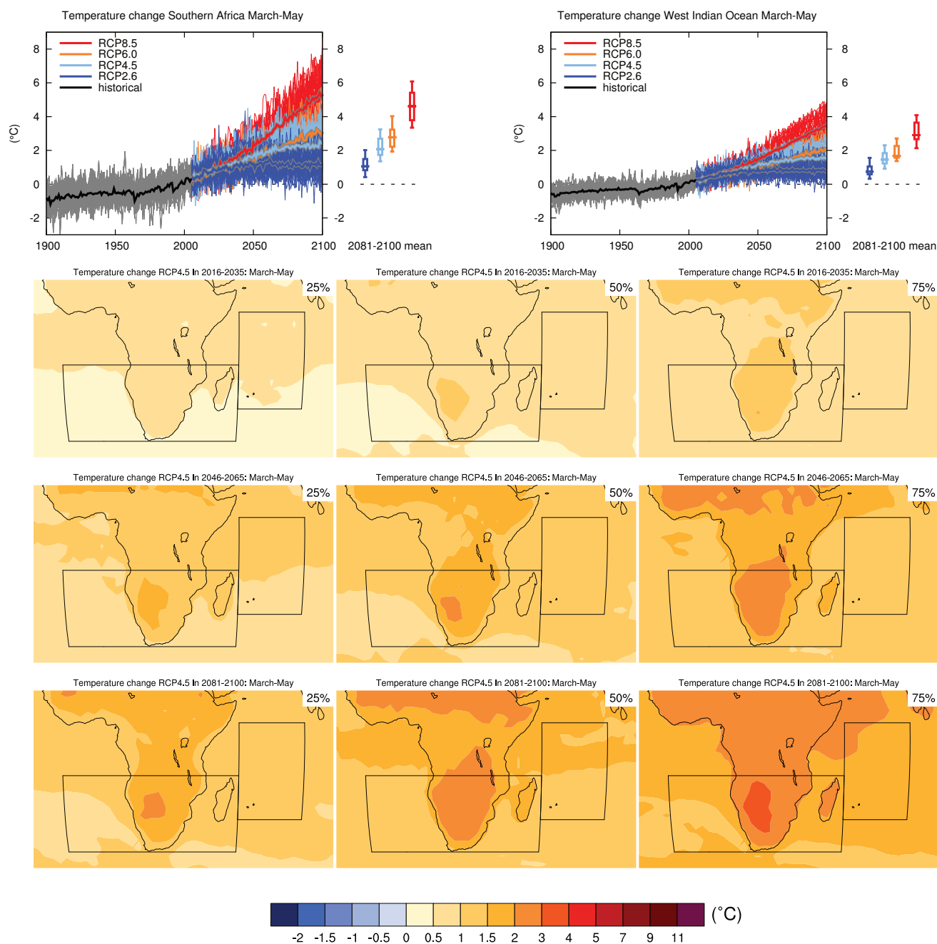
Figure AI.SM4.5.94 | (Top left) Time series of temperature change relative to 1986–2005 averaged over land grid points in Southern Africa (35°S to 11.4°S, 10°W to 52°E) in March to May. (Top right) Same for sea grid points in the West Indian Ocean (25°S to 5°N, 52°E to 75°E). Thin lines denote one ensemble member per model, thick lines the CMIP5 multi-model mean. On the right-hand side the 5th, 25th, 50th (median), 75th and 95th percentiles of the distribution of 20-year mean changes are given for 2081–2100 in the four RCP scenarios.
