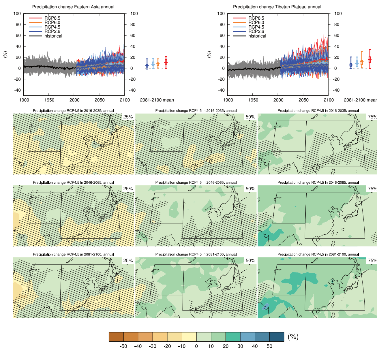
Figure AI.SM4.5.113 | (Top left) Time series of relative change relative to 1986–2005 in annual precipitation averaged over land grid points in Eastern Asia (20°N to 50°N, 100°E to 145°E). (Top right) Same for land grid points on the Tibetan Plateau (30°N to 50°N, 75°E to 100°E). Thin lines denote one ensemble member per model, thick lines the CMIP5 multi-model mean. On the right-hand side the 5th, 25th, 50th (median), 75th and 95th percentiles of the distribution of 20-year mean changes are given for 2081–2100 in the four RCP scenarios.
