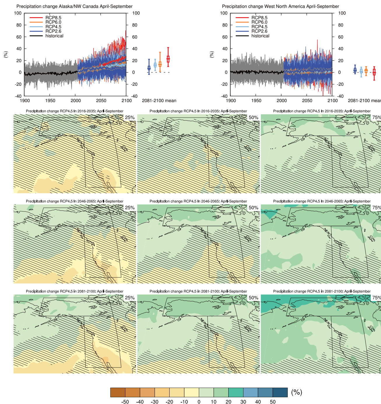
Figure AI.SM4.5.35 | (Top left) Time series of relative change relative to 1986–2005 in precipitation averaged over land grid points in Alaska/NW Canada (60°N to 72.6°N, 168°W to 105°W) in April to September. (Top right) Same for land grid points in West North America (28.6°N to 60°N, 130°W to 105°W). Thin lines denote one ensemble member per model, thick lines the CMIP5 multi-model mean. On the right-hand side the 5th, 25th, 50th (median), 75th and 95th percentiles of the distribution of 20-year mean changes are given for 2081–2100 in the four RCP scenarios.
