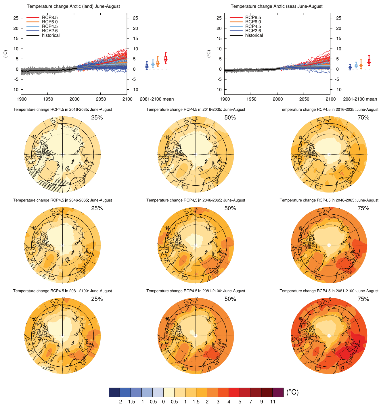
Figure AI.SM4.5.15 | (Top left) Time series of temperature change relative to 1986–2005 averaged over land grid points in the Arctic (67.5°N to 90°N) in June to August. (Top right) Same for sea grid points. Thin lines denote one ensemble member per model, thick lines the CMIP5 multi-model mean. On the right-hand side the 5th, 25th, 50th (median), 75th and 95th percentiles of the distribution of 20-year mean changes are given for 2081–2100 in the four RCP scenarios.
