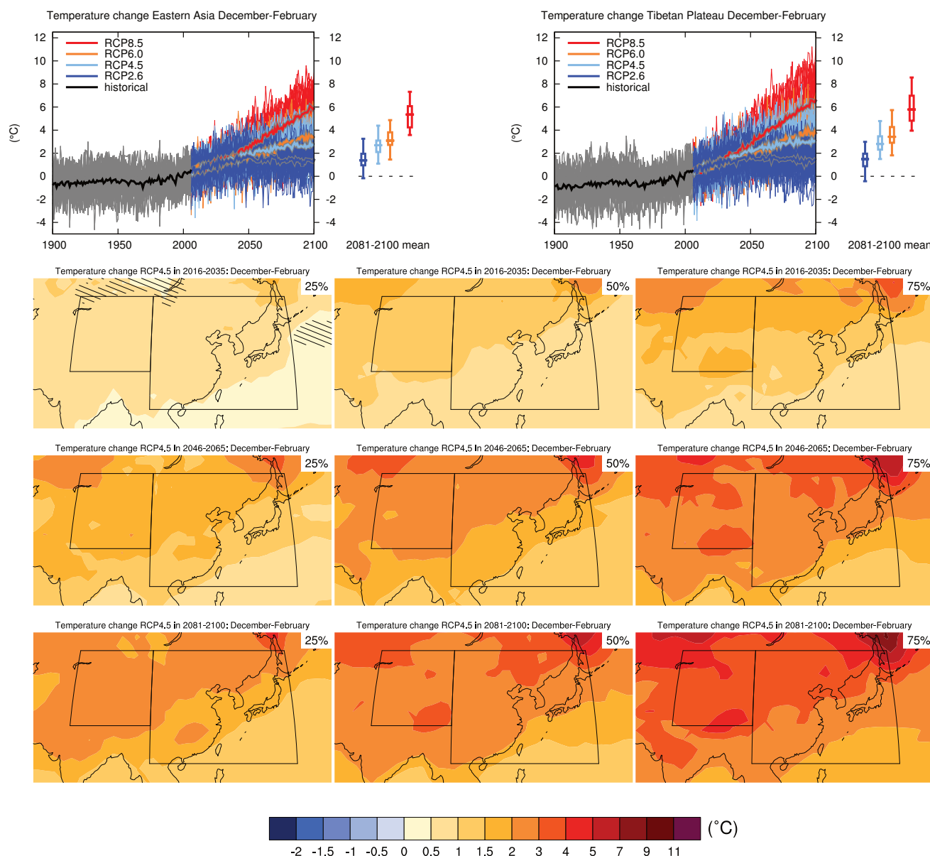
Figure AI.SM4.5.109 | (Top left) Time series of temperature change relative to 1986–2005 averaged over land grid points in Eastern Asia (20°N to 50°N, 100°E to 145°E) in December to February. (Top right) Same for land grid points on the Tibetan Plateau (30°N to 50°N, 75°E to 100°E). Thin lines denote one ensemble member per model, thick lines the CMIP5 multi-model mean. On the right-hand side the 5th, 25th, 50th (median), 75th and 95th percentiles of the distribution of 20-year mean changes are given for 2081–2100 in the four RCP scenarios.
