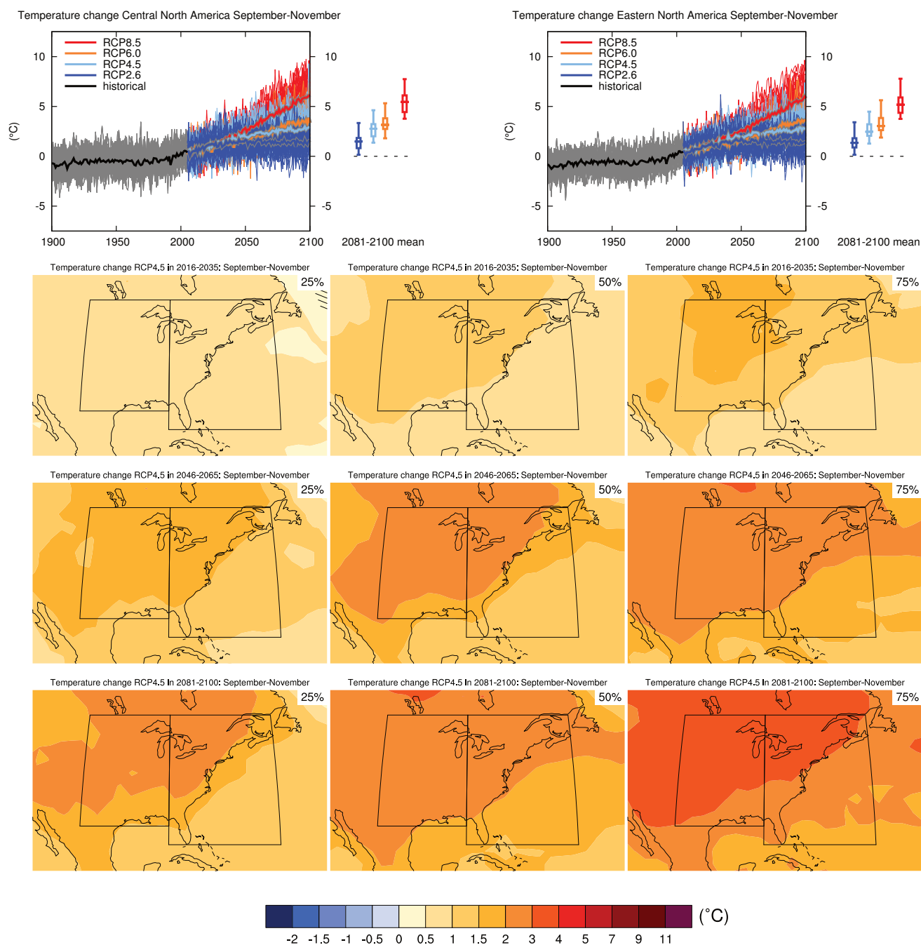
Figure AI.SM4.5.40 | (Top left) Time series of temperature change relative to 1986–2005 averaged over land grid points in Central North America (28.6°N to 50°N, 105°W to 85°W) in September to November. (Top right) Same for land grid points in Eastern North America (25°N to 50°N, 85°W to 60°W). Thin lines denote one ensemble member per model, thick lines the CMIP5 multi-model mean. On the right-hand side the 5th, 25th, 50th (median), 75th and 95th percentiles of the distribution of 20-year mean changes are given for 2081–2100 in the four RCP scenarios.
