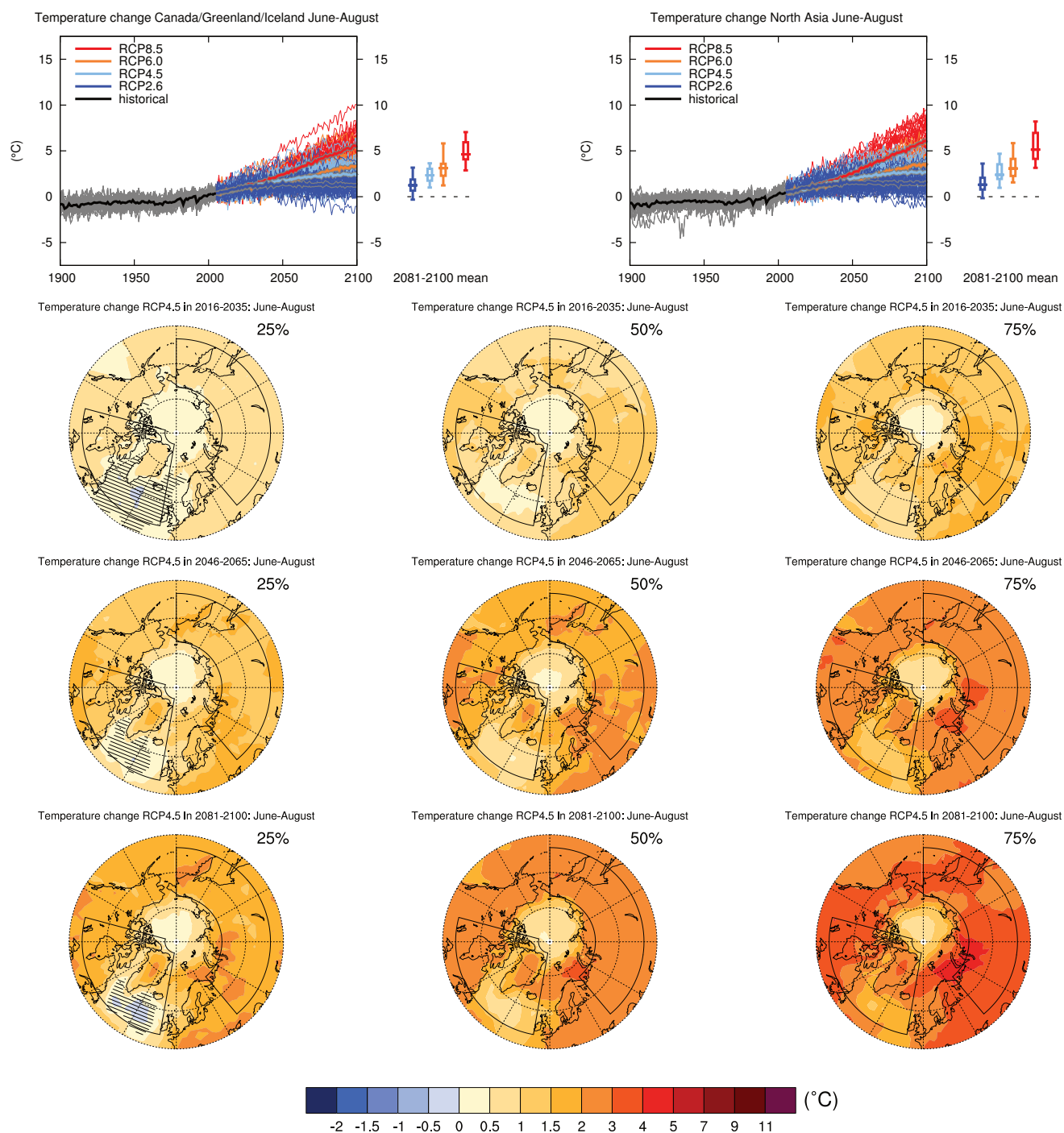
Figure AI.SM4.5.23 | (Top left) Time series of temperature change relative to 1986–2005 averaged over land grid points in Canada/Greenland/Iceland (50°N to 85°N, 105°W to 10°W) in June to August. (Top right) Same for land grid points in North Asia (50°N to 70°N, 40°E to 180°E). Thin lines denote one ensemble member per model, thick lines the CMIP5 multi-model mean. On the right-hand side the 5th, 25th, 50th (median), 75th and 95th percentiles of the distribution of 20-year mean changes are given for 2081–2100 in the four RCP scenarios.
