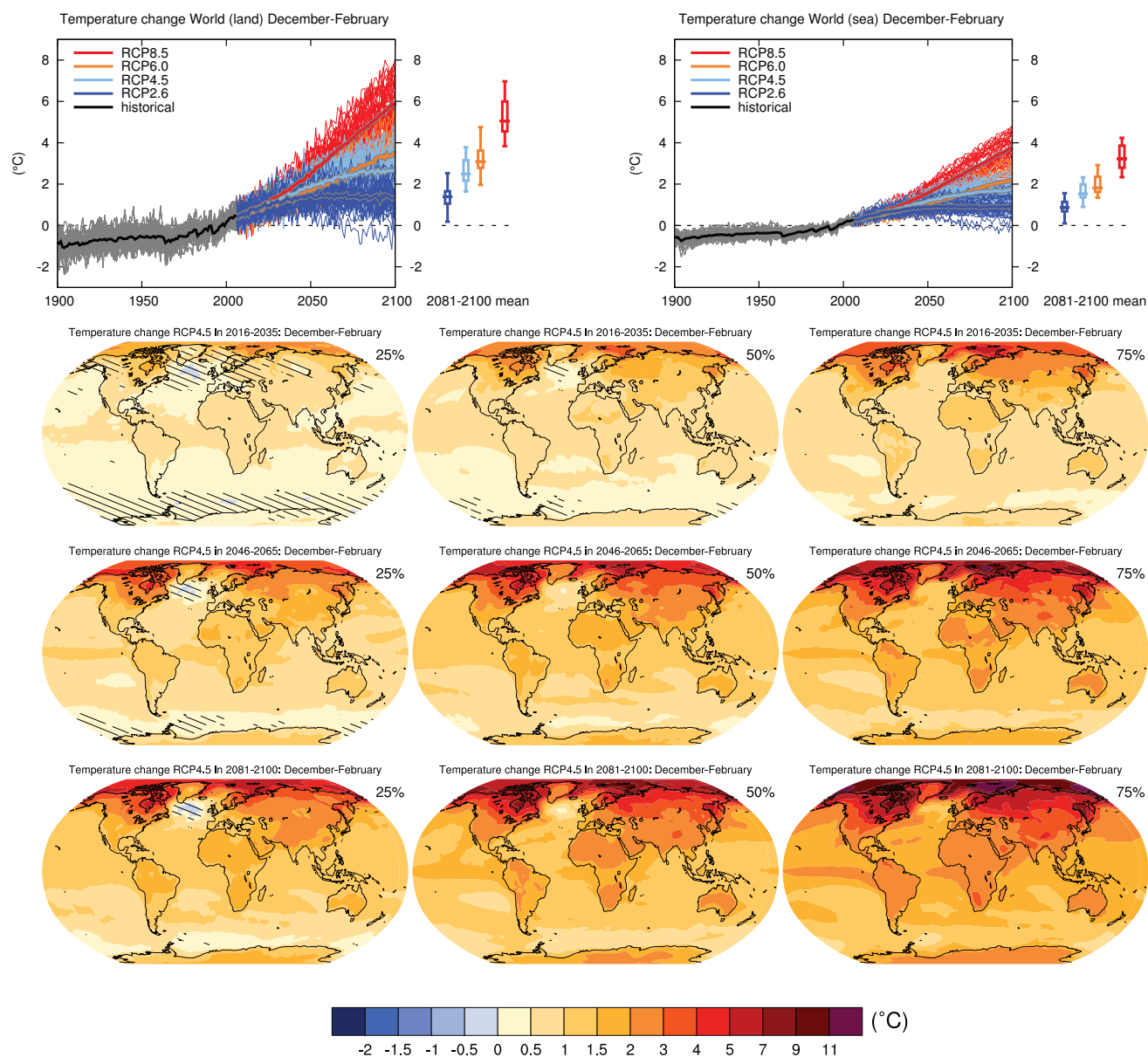
Figure AI.SM4.5.5 | (Top left) Time series of temperature change relative to 1986–2005 averaged over land grid points over the globe in December to February. (Top right) Same for sea grid points. Thin lines denote one ensemble member per model, thick lines the CMIP5 multi-model mean. On the right-hand side the 5th, 25th, 50th (median), 75th and 95th percentiles of the distribution of 20-year mean changes are given for 2081–2100 in the four RCP scenarios.
