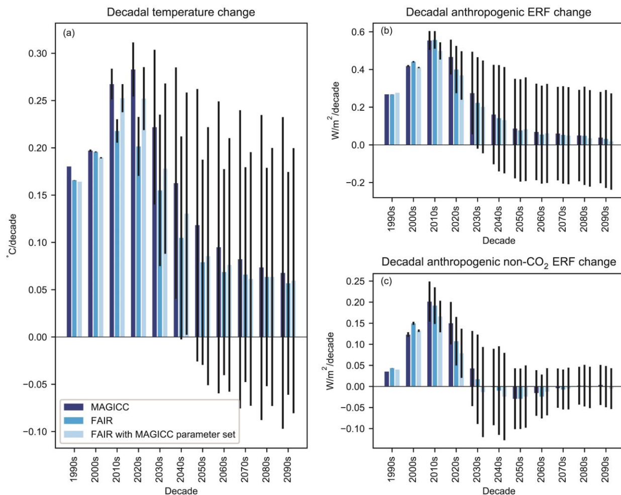
Figure 2.SM.1: Warming rates per decade for MAGICC (dark blue), FAIR (sky blue) and FAIR matching the MAGICC parameter set (light blue) for the scenario dataset used in this report. These bars represent the mean of regression slopes taken over each decade (years 0 to 9) for scenario median temperature changes, over all scenarios. The black bars show the standard deviation over the set of scenarios.
