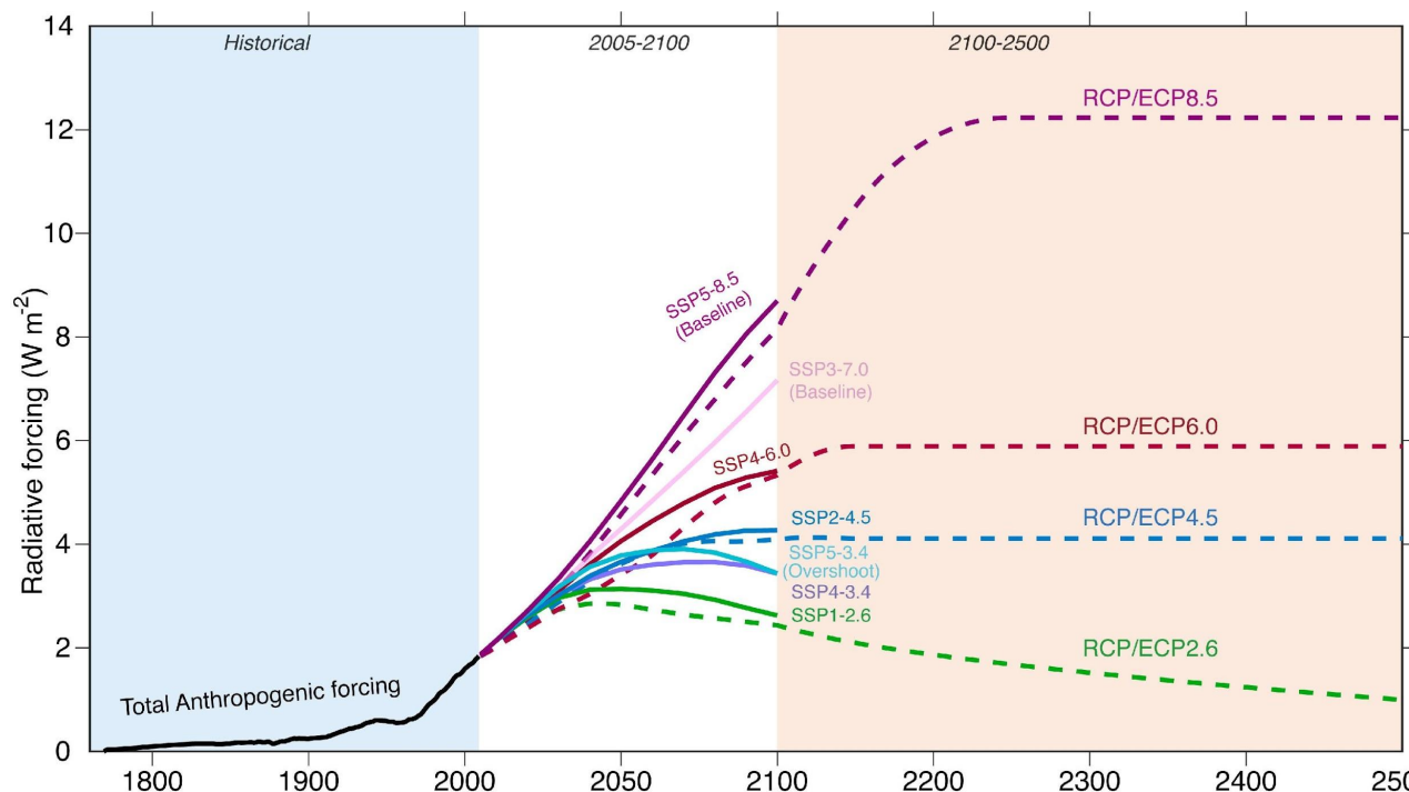
Figure SM1.1: Radiative forcing ( W m^{-2} ) time series for historical data (1765–2004), and for future scenarios from the Representative Concentration Pathways (RCP; 2005–2100) and their continuation as the extended RCPs (2100–2500), and the Shared Socio-economic Pathways (SSP; 2005–2100). The RCP scenarios are shown as dashed curves, and SSPs are shown as solid curves ('Marker' scenarios are used). Note the change in x-axis scale for the 2005–2100 interval to give an improved illustration of radiative forcing scenarios during the 21st century.
